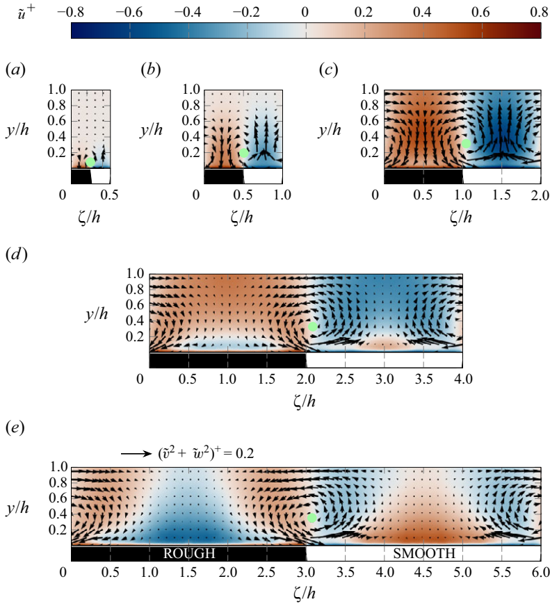
Figure 4. Dispersive velocity field at the initial steady state ( t=0 ) divided in its streamwise \tilde{u}^+ (colour) and circulatory \tilde{v}^+ - \tilde{w}^+ (arrows) patterns; all data at Re_\tau = 500 : (a) \Lambda_s/h = 0.5 ; (b) \Lambda_s/h = 1 ; (c) \Lambda_s/h = 2 ; (d) \Lambda_s/h = 4 ; (e) \Lambda_s/h = 6 . The arrow length is proportional to the magnitude of the represented vector; the scale is graphically represented above panel (e) and is consistent across all panels. Below each panel, we indicate whether the wall at that spanwise position is rough (black) or smooth (white). A green dot marks the position of the vortex centre as defined later in § 5.1.
