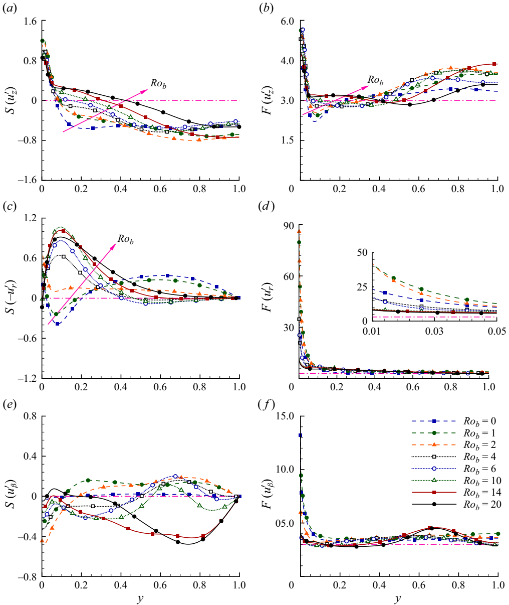
Figure 15. Profiles of skewness ( a,c,e ) and flatness factors ( b,d,f ) of three velocity fluctuations at various rotation numbers of Ro_b = 0\text{--}20 : ( a ) S(u'_z) ; ( b ) F(u'_z) ; ( c ) S(-u'_r) ; ( d ) F(u'_r) ; ( e ) S(u'_\beta) ; ( f ) F(u'_\beta) . The pink dash-dotted line indicates the theoretical values of an ideal Gaussian distribution, which are 0 and 3 for skewness and flatness, respectively. The pink arrow shows a local trend of an increasing rotation number Ro_b . Results are based on test cases of the longest pipes at corresponding rotation numbers listed in table 1 .
