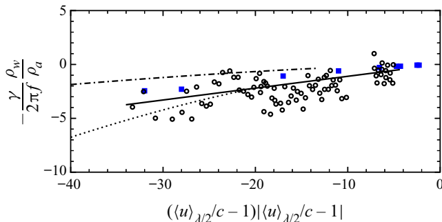
FIGURE 19. Comparison of wave attenuation rate as a function of (u_{\lambda/2}/c - 1)|u_{\lambda/2}/c - 1| between the present LES results and the previous studies. The filled squares (■) and open circles (○) denote the present LES results and the measurement by Donelan (1999), respectively. The solid line (—) is the parameterization of Donelan (1999) -\gamma/(2\pi f) = -0.11\rho_a/\rho_w|u_{\lambda/2}/c - 1|^2 . The dotted (⋯) and dashed-dot (-·-) lines are the parameterization of Peirson et al. (2003) \gamma/f = 2.36 \times 10^{-4}(ak)^{0.240}|u_{\lambda/2}/c - 1|^{3.265} with ak = 0.08 and the parameterization of Mitsuyasu & Yoshida (2005) \gamma/f = 5.8 \times 10^{-5}|u_{\lambda/2}/c - 1|^{3.3} , respectively.
