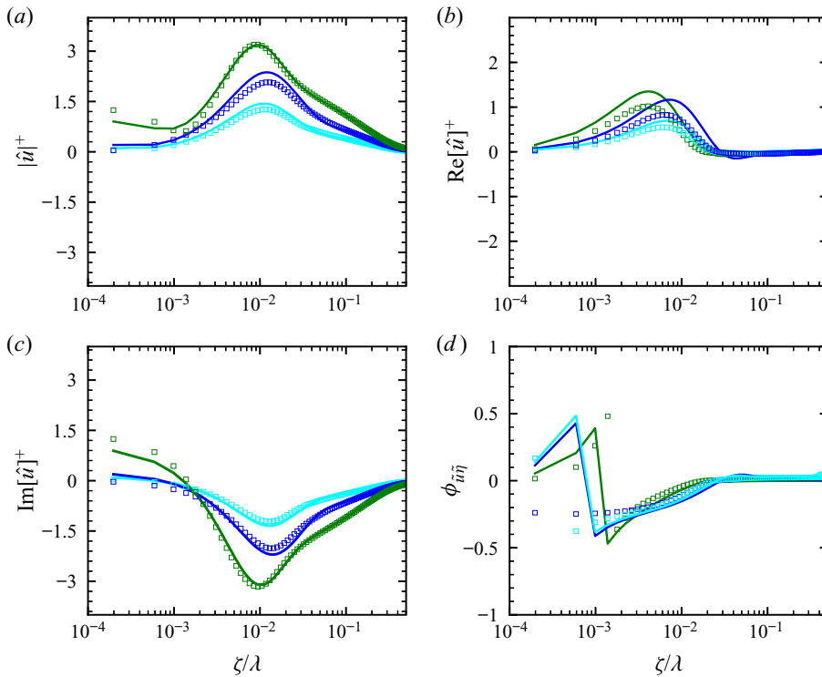
FIGURE 15. Comparison of (a) |\hat{u}|^+ , (b) \text{Re}[\hat{u}]^+ , (c) \text{Im}[\hat{u}]^+ and (d) \phi_{\tilde{u}\tilde{\eta}} between the LES results: WOW01 (—), WOW01L (---) and WOW04 (—); and the solutions of the viscous linearised equation (4.12): WOW01 ( \square ), WOW01L ( \square ) and WOW04 ( \square ). The superscript ‘+’ denotes normalisation by u_\tau .
