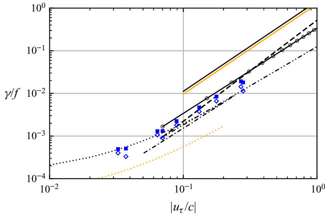
FIGURE 18. Comparison of non-dimensional wave attenuation rate \gamma/f as a function of the inverse wave age |u_\tau/c| between the present and previous studies. The filled squares ( \blacksquare ) and open diamonds ( \diamond ) denote the LES results and the solutions of the viscous linearised equation (4.12), respectively. The dotted lines are the results of Young & Sobey (1985) \gamma/f = 1.4\pi(ak)^2\rho_a/\rho_w(1 - U_\infty/c)^2 with ak = 0.15 (.....) and ak = 0.08 (.....), where U_\infty \approx 30u_\tau in their study. The dash-dot (-.-) and dash-dot-dot (-.-.-) lines show the results of Harris et al. (1995) and Cohen (1997), respectively. The solid lines are the parameterization of Peirson et al. (2003) \gamma/f = 2.275(ak)^{0.238}|u_\tau/c|^{2.112} with ak = 0.15 (—) and ak = 0.08 (—). The parameterization of Mitsuyasu & Yoshida (2005) \gamma/f = 0.52|u_\tau/c|^{2.37} is plotted with the dashed line (- - -). As a reference, the parameterization of wave growth rate in the following wind \gamma/f = 0.34(u_\tau/c)^2 by Mitsuyasu & Honda (1982) is shown using the line with circles ( \circ —).
