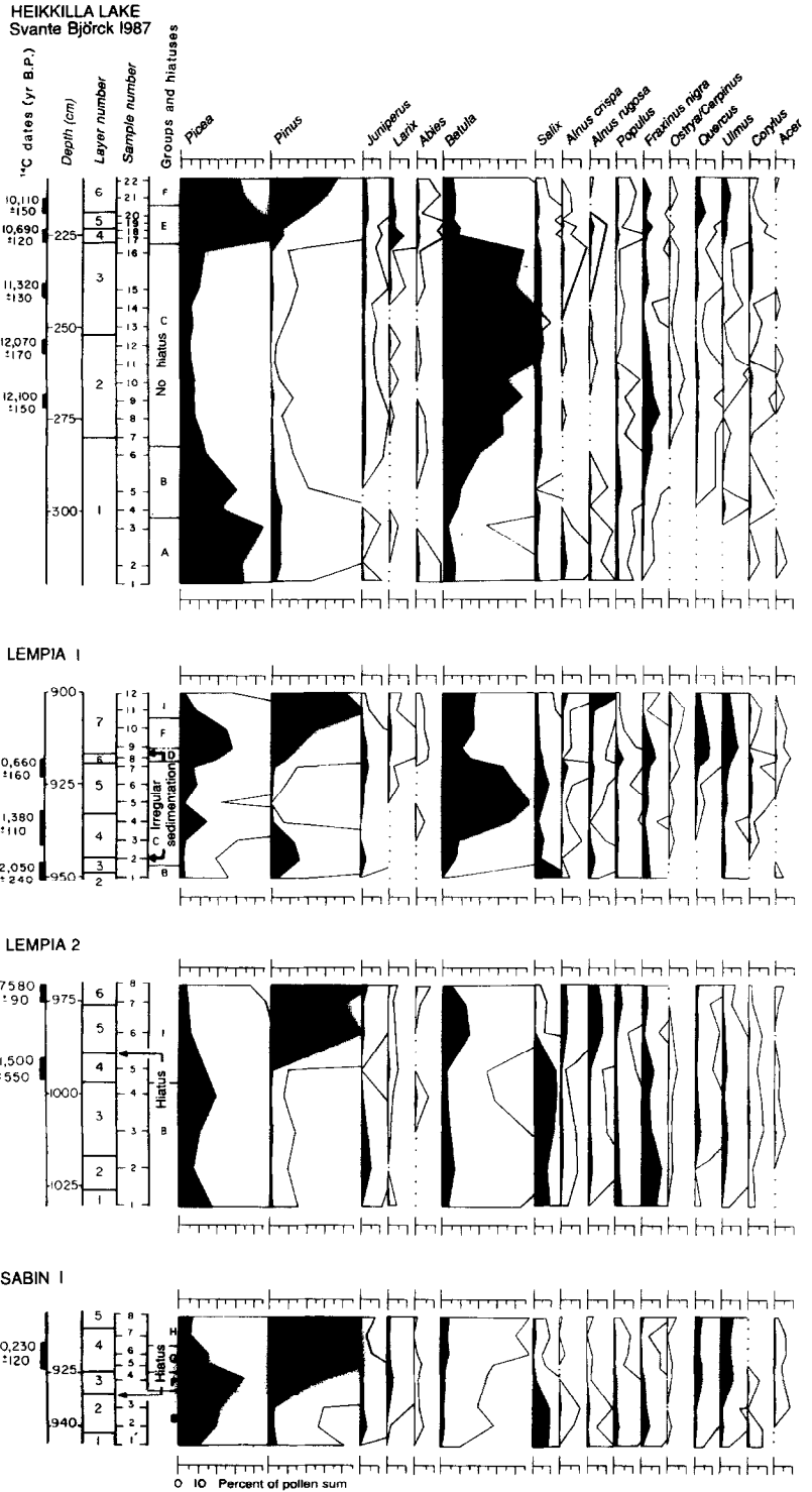
FIG. 7. Pollen diagrams for Heikkilla Lake (No. 1 in Fig. 2), S. Lempia Lake 1 (No. 2 in Fig. 2), S. Lempia Lake 2 (No. 2 in Fig. 2), and Sabin Lake 1 (No. 4 in Fig. 2).
