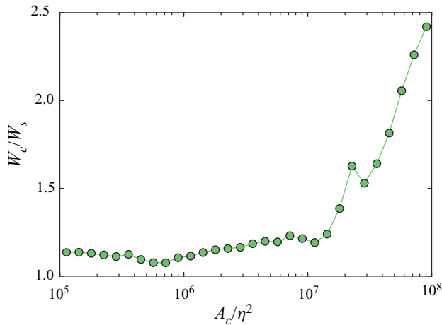
Figure 14. Normalized cluster velocity as a function of cluster size.
