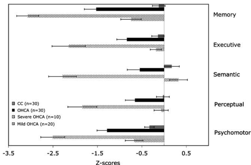
Fig. 1. Composite Z-scores – mean and standard deviation – for controls, all out of hospital cardiac arrest (OHCA), and mild and severe OHCA separately. CC = cardiac control group.
