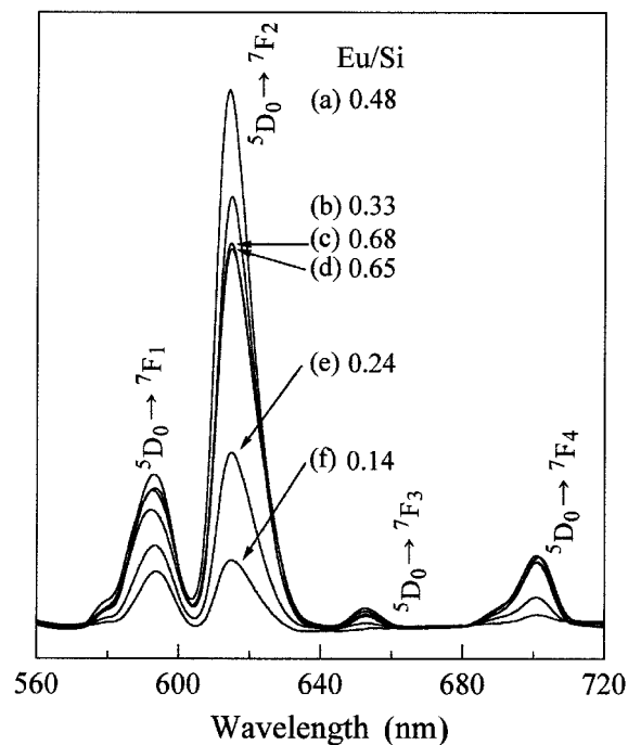
Figure 2. Luminescence spectra of Eu 3+ -magadiites. Eu/Si = 0.48 (a), 0.33 (b), 0.68 (c), 0.65 (d), 0.24 (e) and 0.14 (f).
