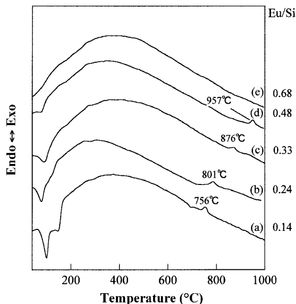
Figure 5. DTA curves of \text{Eu}^{3+} -magadiites. \text{Eu}/\text{Si} = 0.14 (a), 0.24 (b), 0.33 (c), 0.48 (d) and 0.68 (e).
