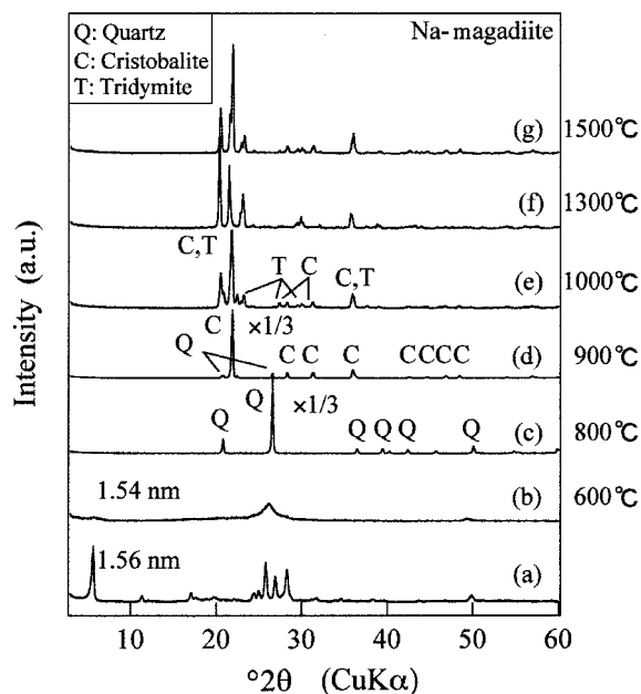
Figure 6. Powder XRD patterns of Na-magadiite before (a) and after the heat treatment at 600 (b), 800 (c), 900 (d), 1000 (e), 1300 (f) and 1500^\circ\text{C} (g).
