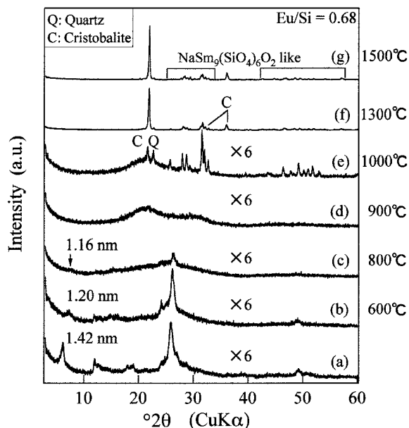
Figure 9. Powder XRD patterns of \text{Eu}^{3+} -magadiite ( \text{Eu/Si} = 0.68 ) before (a) and after the heat treatment at 600 (b), 800 (c), 900 (d), 1000 (e), 1300 (f) and 1500°C (g).
