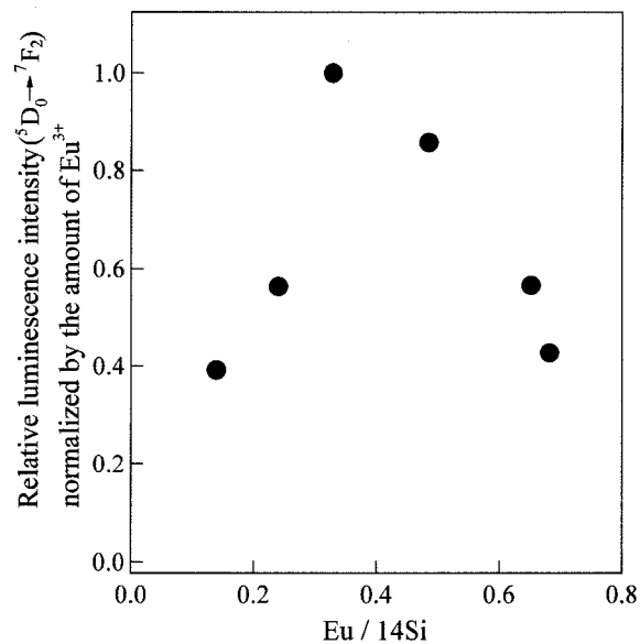
Figure 3. The relationship between the intensity of 5 D 0 - 7 F 2 luminescence band (at 614 nm) and the amount of Eu 3+ adsorbed.
