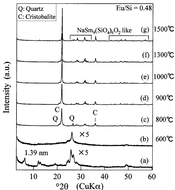
Figure 8. Powder XRD patterns of \text{Eu}^{3+} -magadiite ( \text{Eu/Si} = 0.48 ) before (a) and after the heat treatment at 600 (b), 800 (c), 900 (d), 1000 (e), 1300 (f) and 1500°C (g).
