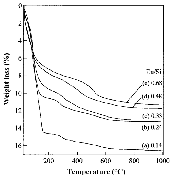
Figure 4. TG curves of \text{Eu}^{3+} -magadiites. \text{Eu}/\text{Si} = 0.14 (a), 0.24 (b), 0.33 (c), 0.48 (d) and 0.68 (e).
