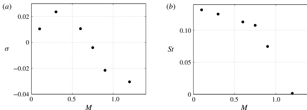
FIGURE 14. Hopf bifurcation. Mach evolution of the (a) temporal amplification rate and (b) Strouhal number for the least temporally damped/most temporally amplified oscillatory global mode at Re = 280 .
