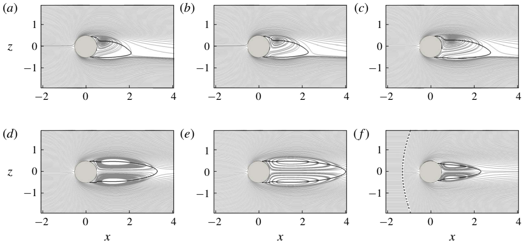
FIGURE 12. Base flow Mach evolution at Re = 280 . Three-dimensional streamlines projected onto the x - z plane for the (a) M = 0.1 , (b) M = 0.3 , (c) M = 0.6 , (d) M = 0.75 , (e) M = 0.9 and (f) M = 1.2 cases. The separated region is indicated by the solid black line. For the supersonic case, the shock is represented by the dashed black line.
