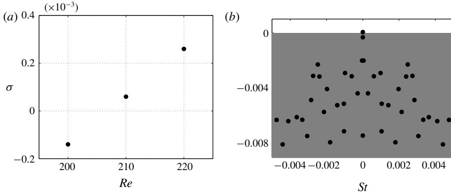
FIGURE 4. Regular bifurcation: (a) temporal amplification rate versus the Reynolds number for the least temporally damped/most temporally amplified non-oscillatory global mode; (b) flow case at Re = 210 ; eigenspectrum in the St - \sigma plane.
