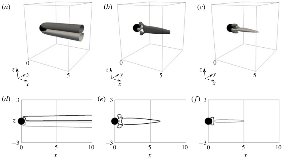
FIGURE 5. Flow case at Re = 210 for the unstable axisymmetric base flow. Three-dimensional view of the mode at (\sigma, St) = (0.683 \times 10^{-4}, 0.0) . The iso-surfaces of the (a) streamwise, (b) radial and (c) azimuthal perturbation velocities are plotted for the levels v'_x = \pm 0.01 , v'_r = \pm 0.01 and v'_\theta = \pm 0.005 , respectively. The contours of the (d) streamwise, (e) radial and (f) azimuthal perturbation velocities are plotted on the x - z plane for the levels v'_x = \pm 0.01 , v'_r = \pm 0.01 and v'_\theta = \pm 0.005 , respectively. Light and dark grey colours for positive and negative perturbation velocities, respectively. The sphere is represented in black.
