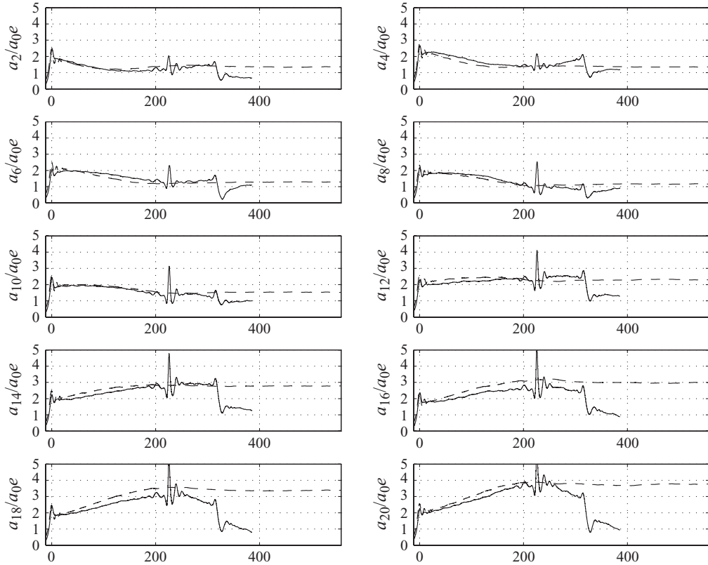
FIGURE 17. Wave period 1.13 s. Steepness H/L = 2\% . Time evolutions of the free-surface elevations RAOs at every other gauge from measurements (solid line) and the Boussinesq model (dashed line).
