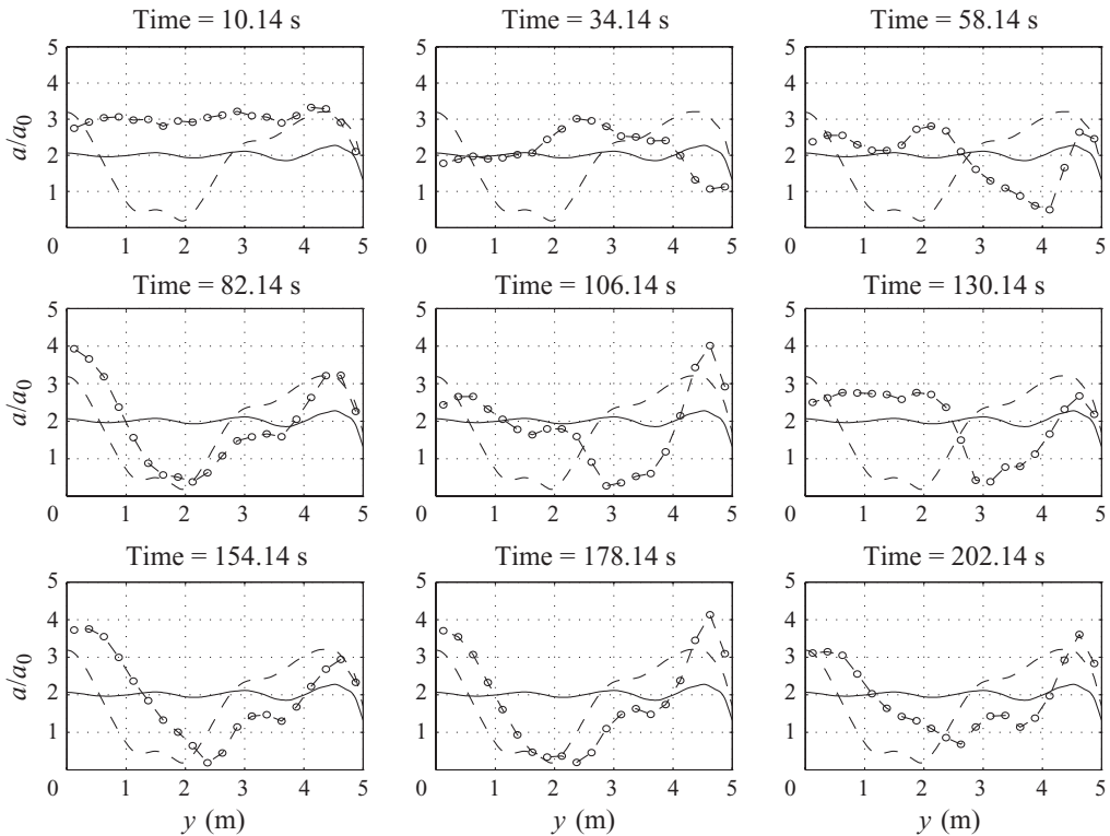
FIGURE 11. Wave period 1.01 s. Steepness H/L = 3.5\% . Time evolution of the free-surface elevation RAO along the plate, from experiments (○), linear theory (solid line) and the parabolic model (dashed line).
