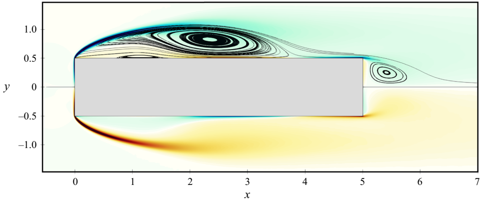
Figure 2. Mean streamlines (top half only) plotted over a colour contour of the mean spanwise vorticity \Omega_z (blue/red indicates negative/positive values in the range -20 \leq \Omega_z \leq 20 ).
