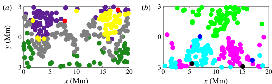
FIGURE 14. K -means clustering of the Bickley jet with 480 randomly initialized particles; five of the 10 total clusters identified are shown in (a) and the remaining five in (b).
