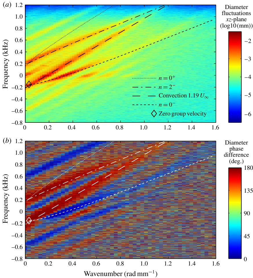
FIGURE 10. Wavenumber–frequency amplitude (a) and phase spectrum (b) at the condition of figure 6(b). Included are the lines for the breathing n=0^\pm and helical n=2^\pm modes and a line for constant group velocity that is 19% larger than the tunnel free stream velocity. Derived quantities; \Omega = 2.0 \times 10^3 \text{ rad s}^{-1} , r_c = 2.3 \text{ mm} , r_v = 1.9 \text{ mm} and \Gamma = 0.10 \text{ m}^2 \text{ s}^{-1} .
