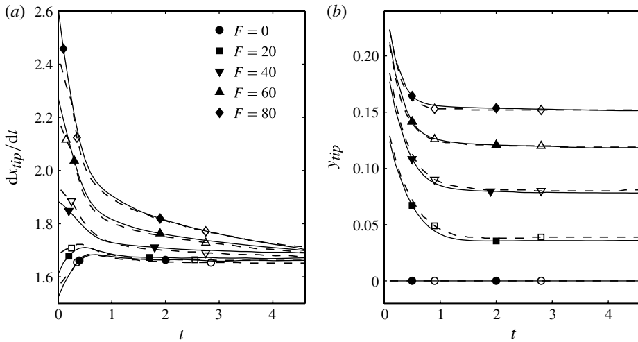
FIGURE 3. Velocity of the front dx_{tip}/dt and front elevation y_{tip} (—) as a function of time for various F , R = 2.5 , Pe = 2000 and Re = e^{-2.5} . The Stokes flow results of Talon et al. (2013) are shown for comparison (---).
