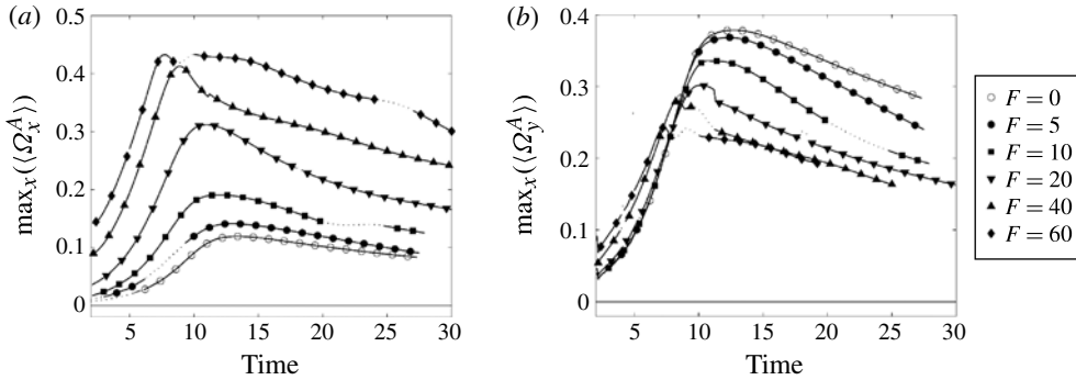
FIGURE 24. Maximum values (—), and interpolated curves ( \cdot \cdot \cdot ): (a) streamwise vorticity component \max_x(\langle |\Omega_x| \rangle_{y,z}^A(F, t)) ; (b) gapwise vorticity component \max_x(\langle |\Omega_y| \rangle_{y,z}^A(F, t)) for various F , R = 2.0 , Re = e^{-2.0} and Pe = 2000 .
