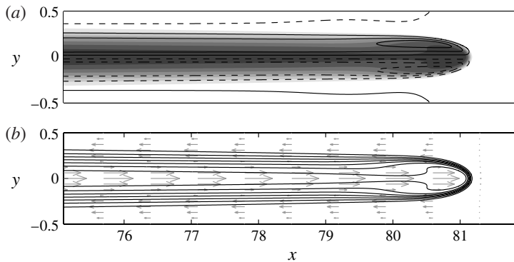
FIGURE 5. Dispersive pinch-off of the concentration contours immediately behind the finger tip. (a) Concentration field ( \Delta c = 0.1 ) in grey levels and contour lines of vorticity after the base Poiseuille flow has been subtracted out. Positive vorticity is represented by continuous lines and negative vorticity by dashed ones. (b) Black contours show the concentration field and grey arrows represent the velocity field, after the base Poiseuille flow has been subtracted out. Time t = 50 , the parameter values are F = 0 , R = 2.0 , Re = e^{-2.0} and Pe = 2000 . Here, the c = 0.2 contour has already pinched off, and the c = 0.3 contour is about to pinch off near x = 80 , cf. also figure 8 for the pinch-off times of the concentration contours.
