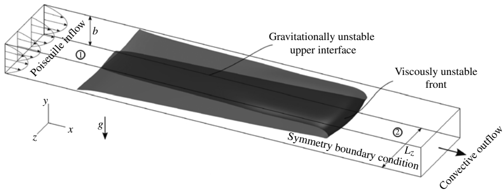
FIGURE 1. Schematic figure showing the problem geometry: injected fluid 1 ( \mu_1, \rho_1, c = 0 ) displaces resident fluid 2 ( \mu_2 > \mu_1, \rho_2 > \rho_1, c = 1 ) in the positive x -direction, driven by Poiseuille inflow. Gravity acts in the negative y -direction. Solid walls form the top and bottom boundaries, while symmetry conditions are assumed at the z -boundaries. The grey surface denotes the c = 0.5 concentration contour, which can be considered a representation of the miscible interface.
