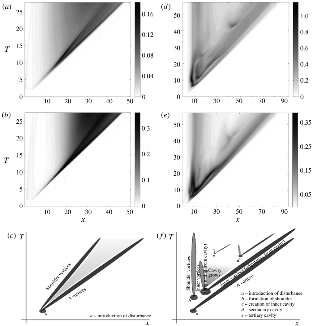
FIGURE 22. Contour plots of the (y, z) -averaged magnitude of the streamwise and gapwise vorticity components, for R = 2.0 , Re = e^{-2.0} , Pe = 2000 and F = 5 ( a – c ) and F = 60 ( d – f ). ( a, d ) Streamwise component \langle |\Omega_x| \rangle_{y,z}(x, t) . ( b, e ) Gapwise component \langle |\Omega_y| \rangle_{y,z}(x, t) . ( c, f ) Schematic representation. By focusing on the locations where the vorticity has a maximum in the (x, t) -plane, it indicates that the pattern formation is associated with the vorticity dynamics.
