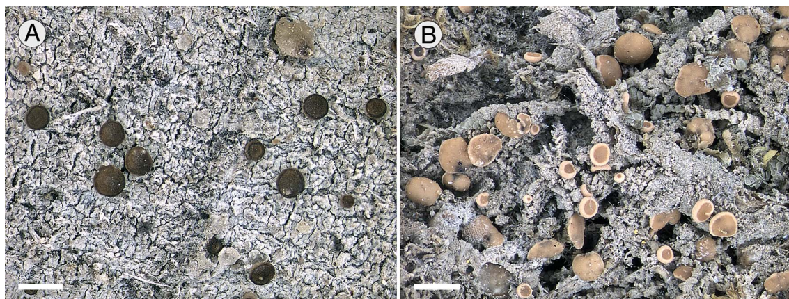
Fig. 3. A, habit of Australidea canorufescens . B, habit of Malcolmiella interversa . Scales = 1 mm. In colour online.
