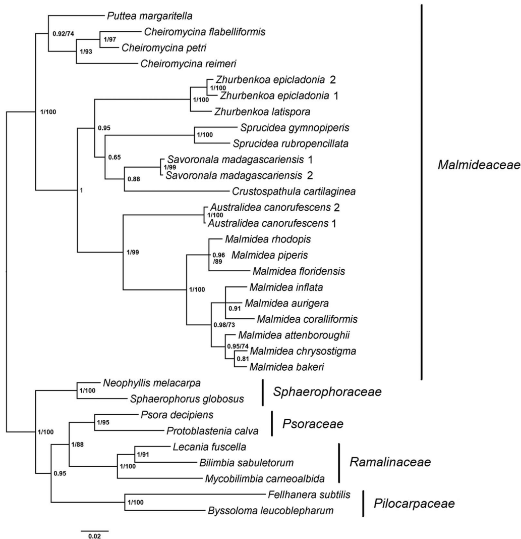
Fig. 1. Majority-rule consensus tree based on a Bayesian MCMC analysis of mrSSU and LSU, showing the phylogenetic position of Australidea in the Malmideaceae. Branch support is given as posterior probability (PP)/bootstrap support (BS). Bootstrap support values are from a corresponding maximum likelihood analysis. Only BS values > 70% are shown. GenBank Accession numbers and voucher information are given in Table 1.
