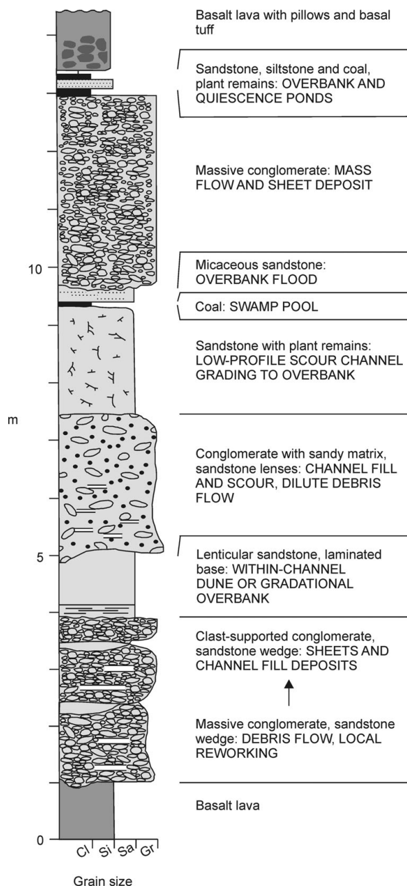
Figure 5. Stratigraphical log for the Allt Geodh' a' Ghamhna Member [NG 3690 1970] of the Minginish Conglomerate Formation, Skye (after Williamson & Bell, 1994).
