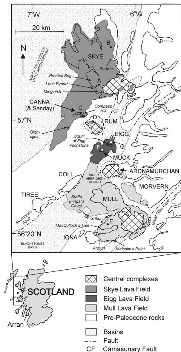
Figure 1. Maps indicating the position of the Paleocene central complexes and lava fields in NW Scotland. A–G – position of sections in Figure 4. NW–SE and NNW–SSE trending dyke swarms omitted for clarity. Structural and basin data after Fyfe, Long & Evans (1993).
