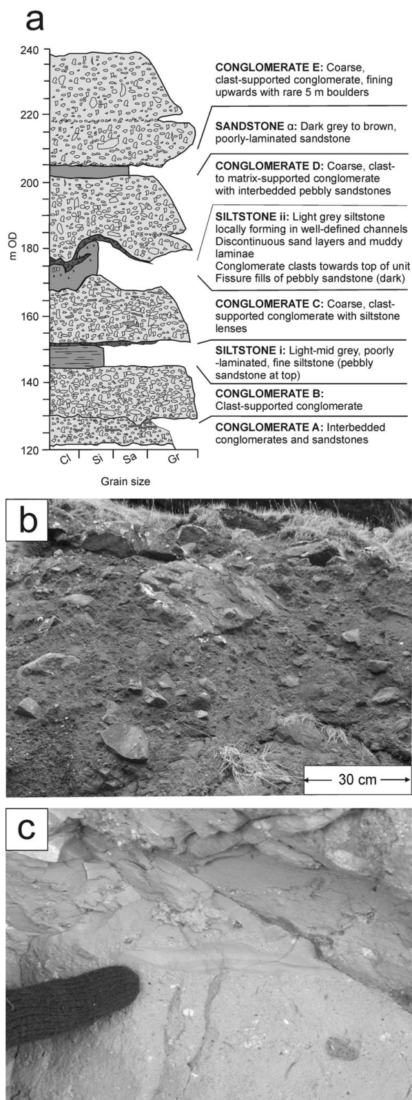
Figure 8. (a) Stratigraphical log located NE of MacLean's Nose, Ben Hiant, Ardnamurchan [NM 5370 6194], depicting strata and characteristics of the Ben Hiant Member. (b) Matrix-supported conglomerate/breccia from Conglomerate B of the Ben Hiant Member. (c) Muddy laminae in Siltstone ii of the Ben Hiant Member.
