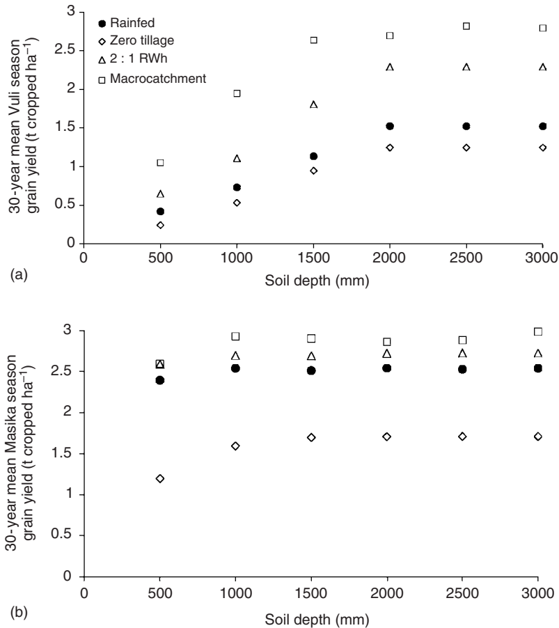
Figure 3. The effects of soil depth on mean maize grain yield in the (a) Vuli and (b) Masika season for each of the four treatments. Results are from 30-year simulations using weather data generated to match that at Kisangara. (Note: maximum rooting depth is set of 1.8 m).
