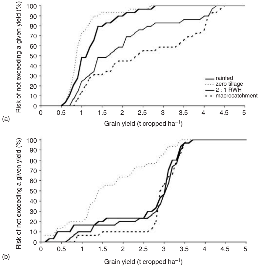
Figure 2. The risk of not exceeding a given maize grain yield in the (a) Vuli and (b) Masika season for each of the four treatments is calculated from 30-year simulations using weather data generated to match that at Kisangara.
