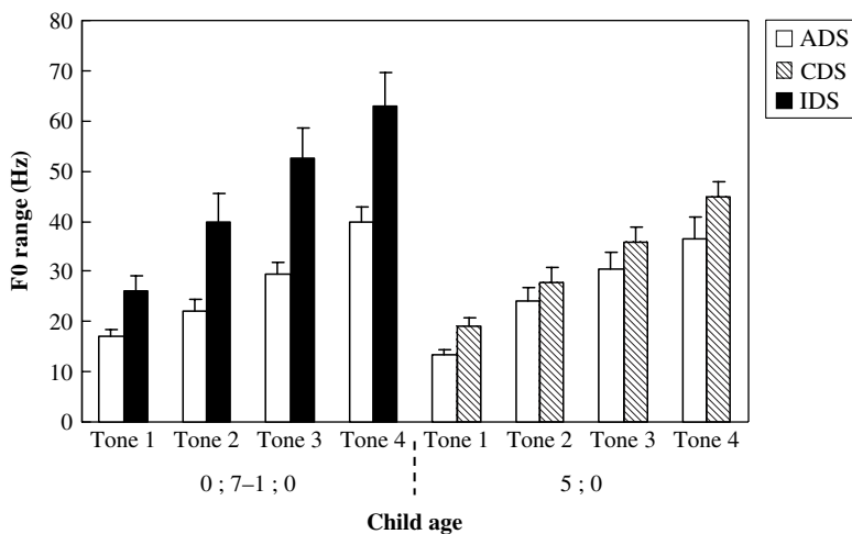
Fig. 2. The F_0 range of four lexical tones in Mandarin ADS, IDS and CDS to children at two ages (SE in error bars).
