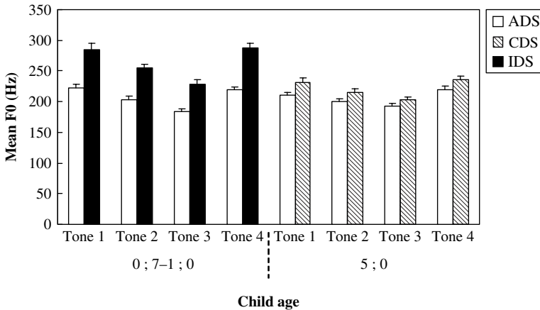
Fig. 1. The mean F_0 values of four lexical tones in Mandarin ADS, IDS and CDS to children at two ages (SE in error bars).
