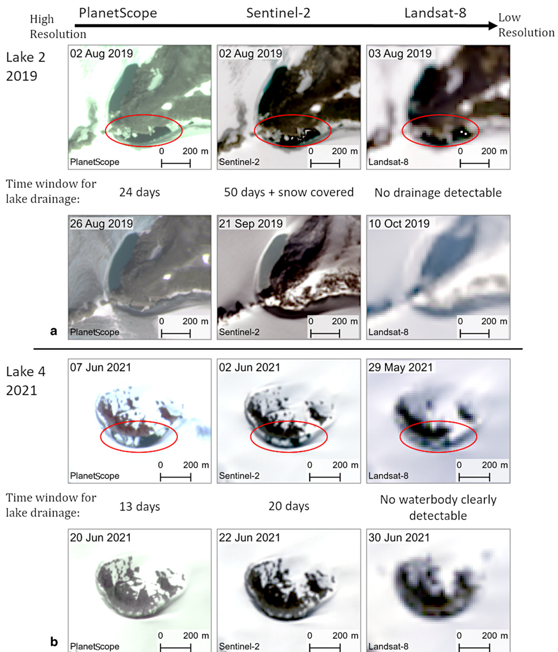
Figure 4. Detectability of Tystigreen's glacial lakes in the PlanetScope (left), Sentinel-2 (middle) or Landsat-8 (right) imagery, including the time window constraining the glacial lake drainages for each satellite product. The upper two panels (a) show an example of the drainage event from lake 2 in 2019. The lower two panels (b) depict the drainage of lake 4 in 2021. Projection: WGS1984 UTM Zone 32N.
