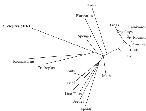
Fig. 2. C. elegans SID-1 is widely conserved. SID-1 homologues are present in many taxonomic groups, suggesting widespread conservation of a protein, which may support systemic RNAi in these other species. The taxonomic tree of C. elegans SID-1 was created using Grishin (protein) distance, with a max sequence difference of 0.85, a fast minimum evolution parameter, and with radial display representing inferred evolutionary distance.
