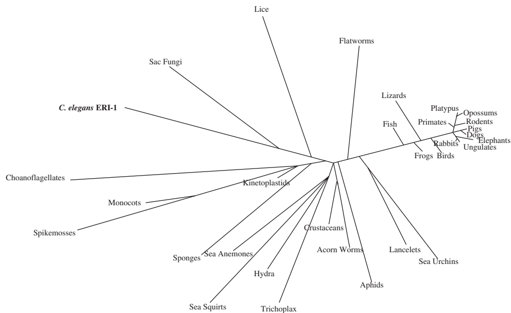
Fig. 5. C. elegans ERI-1 is widely conserved. ERI-1, which is important for the production or stability of endogenous siRNA in C. elegans , has homologues in many taxonomic groups. Since it is likely that endogenous RNAi processes will compete with exogenous RNAi processes in these species, researchers should not only consider the possibility of enhancing RNAi, but the possibility that exogenous RNAi will interfere with essential endogenous processes (e.g. eri-1 and rrf-3 are required for sperm function). The taxonomic tree of C. elegans ERI-1 was created using Grishin (protein) distance, with a max sequence difference of 0.85, a fast minimum evolution parameter, and with a radial display representing inferred evolutionary distance.
