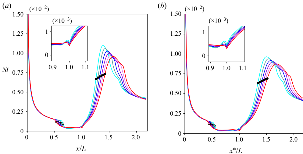
Figure 16. Stanton number distribution at the symmetry plane of the 20° FSM with (a) 40 μm and (b) 200 μm leading-edge bluntness. Cyan, s_w = 0.095 ; blue, s_w = 0.143 ; dark blue, s_w = 0.190 ; dark violet, s_w = 0.238 ; violet, s_w = 0.286 ; red, s_w = 0.333 .
