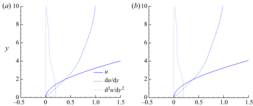
Figure 30. Velocity and derivative profiles for s_w = 0.095 (a) and s_w = 0.333 (b) at reattachment points x = 7.05 and x = 7.92 , for \alpha = 3.72 and \alpha = 4.13 , respectively.
