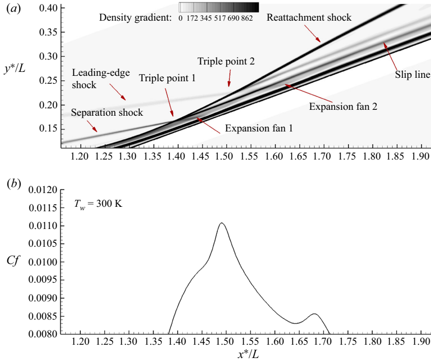
Figure 9. First type of shock interference for the 20^\circ FSM with sharp-leading edge ( 40\ \mu\text{m} ) and T_w = 300 K. Density gradient magnitude contour (a) and skin-friction plot (b) in the shock–shock interaction region.
