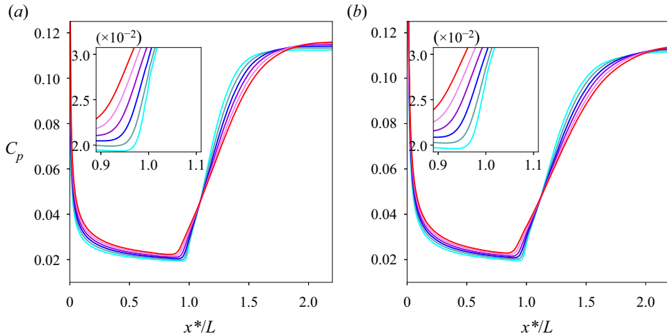
Figure 12. Pressure coefficient distribution at the symmetry plane of the 10^\circ FSM with (a) 40\ \mu\text{m} and (b) 200\ \mu\text{m} leading-edge bluntness. Cyan, s_w = 0.095 ; blue, s_w = 0.143 ; dark blue, s_w = 0.190 ; dark violet, s_w = 0.238 ; violet, s_w = 0.286 ; red, s_w = 0.333 .
