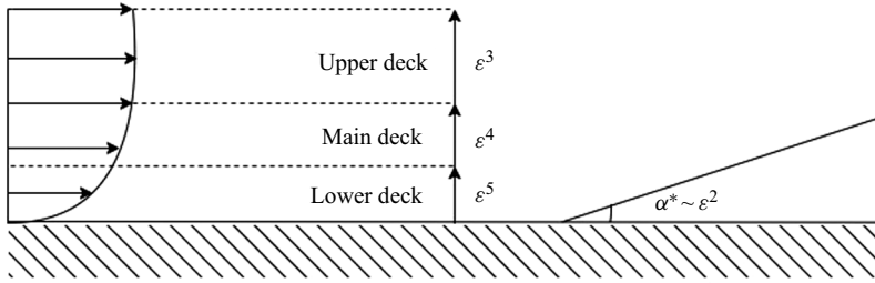
Figure 1. Asymptotic structure of a boundary layer approaching the corner according to the triple-deck theory.
