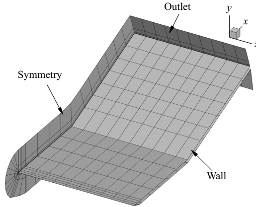
Figure 3. Coarse version of the grid for the FSM with 20° and sharp leading-edge. Some surfaces have been removed for better visualisation.
