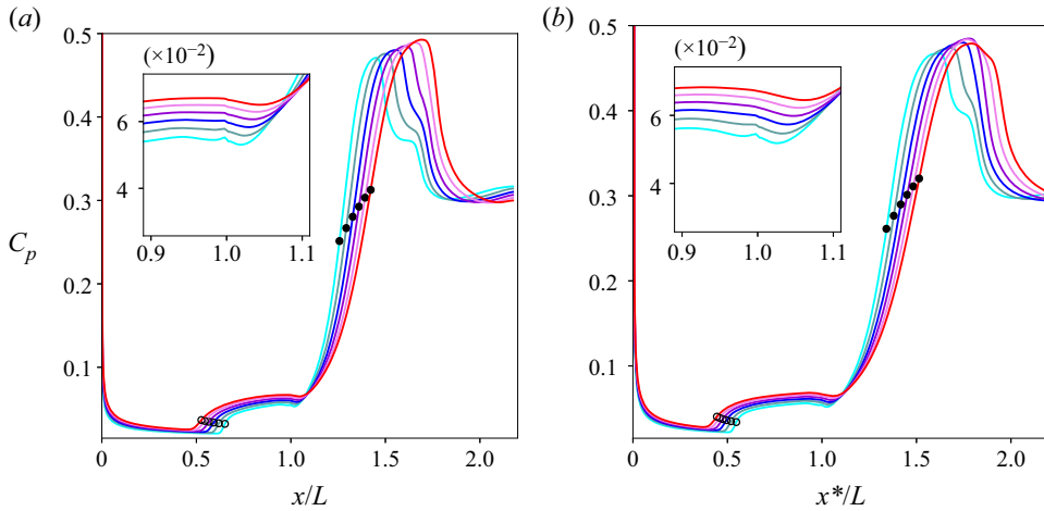
Figure 15. Pressure coefficient distribution at the symmetry plane of the 20° FSM with (a) 40 μm and (b) 200 μm leading-edge bluntness. Cyan, s_w = 0.095 ; blue, s_w = 0.143 ; dark blue, s_w = 0.190 ; dark violet, s_w = 0.238 ; violet, s_w = 0.286 ; red, s_w = 0.333 .
