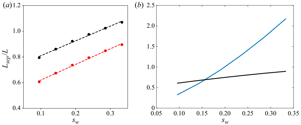
Figure 31. (a) Effect of wall temperature and bluntness on separation length (red, 40 \mu\text{m} ; black, 200 \mu\text{m} ). (b) Comparison of separation length with triple-deck (blue) and N–S (black) solutions.
