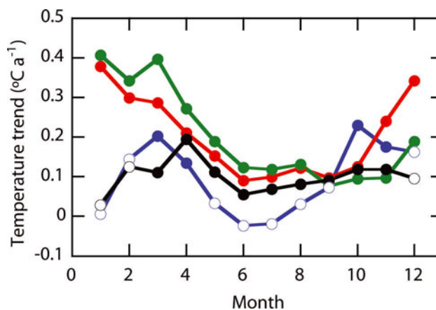
Fig. 6. Temperature trends for 1982–2008 in Pituffik (blue), Kitsissorsuit (red), Nuussuaq (green) and Daneborg (black). Dots are statistically significant at the 90% level, circles are not.
