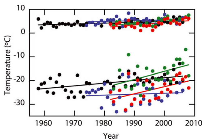
Fig. 5. Monthly-mean temperatures for Pituffik (blue), Kitsissorsuit (red), Nuussuaq (green) and Daneborg (black). High values are July temperatures, low values are February temperatures, and lines are linear fits to the data.
