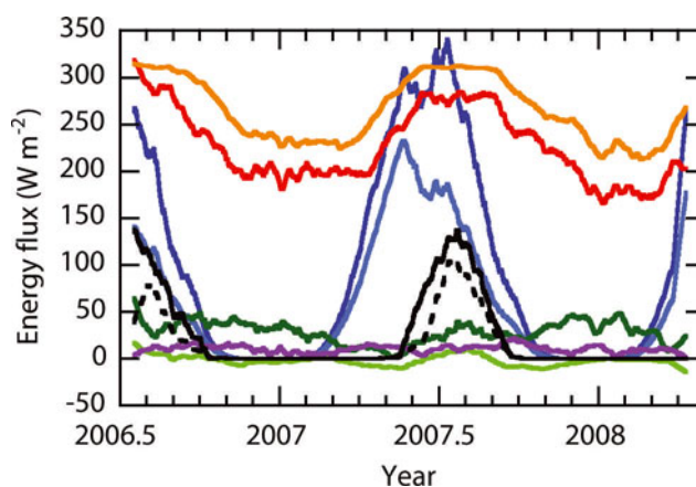
Fig. 12. Thirty-day running mean values of the energy budget components at the AWS on Steenstrup Gletscher: downwelling and reflected shortwave radiation (dark and light blue respectively), absorbed and emitted longwave radiation (red and orange respectively), sensible and latent heat fluxes (dark and light green respectively), subsurface heat flux (purple) and the energy used for melt (black), which is partly within the ice and snow due to shortwave radiation penetration (dotted curve). All fluxes are plotted as gains to the surface budget, except for the outgoing/reflected radiative fluxes and melt, to facilitate visual comparison.
