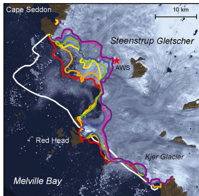
Fig. 2. Modified Landsat image of Steenstrup Gletscher in 1999 showing glacier extent in 1916 (white), 1949 (red), 1963 (orange), 1975 (yellow), 1985 (green), 1999 (blue), 2007 (pink) and 2009 (purple). The white curve is taken from a hand-drawn map by L. Koch. Other curves are based on aerial and satellite imagery. The position of the AWS is marked with a star. See also Dawes and Van As (2010).
