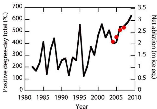
Fig. 7. Yearly PDD totals at Kitsissorsuit (black curve) and measured net ablation on Steenstrup Gletscher (red dots).
