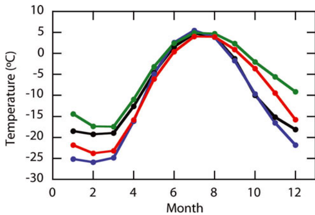
Fig. 4. Mean monthly temperatures as measured by land-based weather stations in Pituffik (blue), Kitsissorsuit (red), Nuussuaq (green) and Daneborg (black) for 1982–2008.
