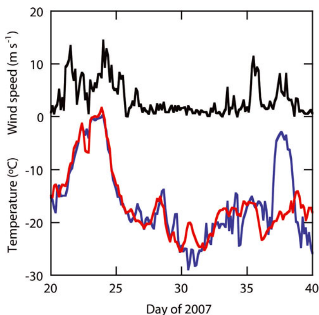
Fig. 9. Three-hourly values of wind speed (black) and temperature (blue) at Steenstrup Gletscher, and temperature at Kitsissorsuit (red).
