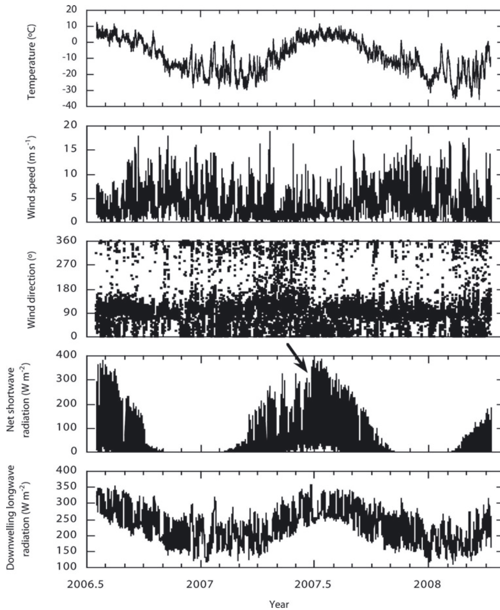
Fig. 10. Hourly values of air temperature, wind speed, wind direction relative to north, net shortwave radiation and downwelling longwave radiation at the AWS on Steenstrup Gletscher. An arrow indicates the transition from a snow surface to an ice surface in 2007.
