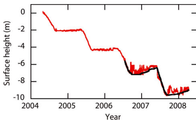
Fig. 11. Measured (red) and modelled (black) surface height change due to ablation and accumulation at the AWS on Steenstrup Gletscher. Note that the measurements do not capture wintertime accumulation.
