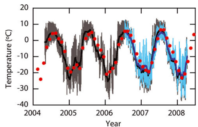
Fig. 8. Hourly (thin bars) and 30 day running mean values (thick curves) of air temperature (light and dark blue) and logger enclosure temperature (grey and black) on Steenstrup Gletscher. Red dots show monthly-mean values at Kitsissorsuit.
