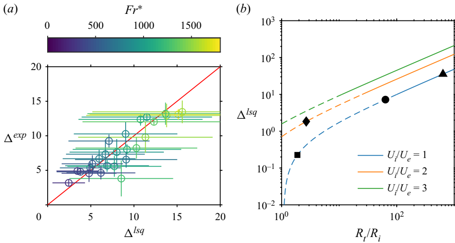
Figure 17. (a) Experimental mass of equilibrated silicates \Delta^{exp} , as a function of the mass of equilibrated silicates scaling \Delta^{lsq} (6.2), using f_m = 1 . Colours scale as the modified Froude number Fr^* . (b) Mass of equilibrated silicates scaling \Delta^{lsq} as a function of the target-to-impactor radius R_t/R_i (6.3), for several impact velocities U_i , and using f_m = 0.16 and \rho_m/\rho_s = 2 . Symbols and lines: triangle, impactor of 10 km in radius onto a Earth-sized target; circle, impactor of 100 km in radius onto a Earth-sized target; square, canonical Moon-forming impact with a Mars-sized impactor (Canup 2004); diamond, fast-spinning Earth Moon-forming impact with a fast ( U_i = 2U_e ) and small ( R_t/R_i = 0.3 ) impactor (Cuk & Stewart 2012); dashed lines correspond to an extrapolated range of Froude number, i.e. Fr < 200 , which is outside of the experimental Froude number range.
