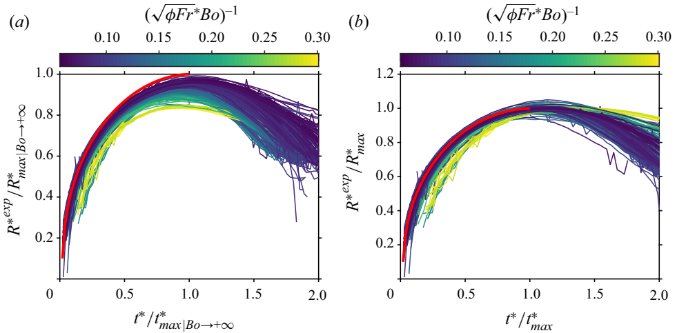
Figure 10. (a) Experimental mean crater radius normalised by the maximum crater radius scaling R^{*exp}/R_{max|Bo \rightarrow +\infty}^* , as a function of time normalised by the crater opening time scaling t^*/t_{max|Bo \rightarrow +\infty}^* , with scaling laws neglecting surface tension. (b) Experimental mean crater radius normalised by the maximum crater radius scaling R^{*exp}/R_{max}^* , as a function of time normalised by the crater opening time scaling t^*/t_{max}^* , with scaling laws including surface tension. The thick solid line corresponds to the solution of (4.8) when 1/(\sqrt{\phi Fr^* Bo}) = 0 , i.e. without surface tension. Colours scale as 1/(\sqrt{\phi Fr^* Bo}) .
