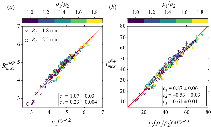
Figure 8. (a) Experimental normalised maximum crater radius R_{max}^{*exp} , as a function of the least squares best-fit power-law scaling R_{max}^{*lsq} (4.15). (b) Experimental normalised crater opening time t_{max}^{*exp} , as a function of the least squares best-fit power-law scaling t_{max}^{*lsq} (4.18). Colours scale as the density ratio \rho_1/\rho_2 . Circles and crosses correspond, respectively, to large and small drop size series.
