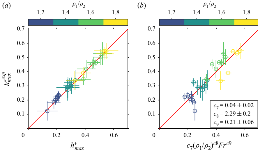
Figure 16. (a) Experimental normalised maximum mixing layer thickness h_{max}^{*exp} as a function of the maximum thickness h_{max}^* predicted by the buoyancy–drag model ((4.8), (5.3) and (5.6)). (b) Experimental normalised maximum mixing layer thickness h_{max}^{*exp} as a function of the least squares best-fit power-law scaling h_{max}^{*lsq} (5.20). Colours scale as the density ratio \rho_1/\rho_2 .
