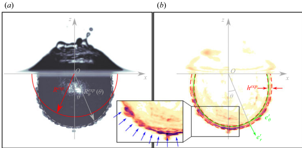
Figure 3. (a) Detection of the crater boundary. The dashed line corresponds to the fitted crater boundary using a set of shifted Legendre polynomials up to degree l = 5 , the degree l = 0 gives the solid line corresponding to the mean crater radius. (b) Detection of the mixing layer. The solid line corresponds to the fitted crater boundary using a set of Legendre polynomials up to degree l = 5 . The dashed lines correspond to the weighted average of the mixing layer boundaries, calculated using the second moment of the LIF intensity about the mean position of the layer. Blue arrows indicate the position of the plumes produced by the instability.
