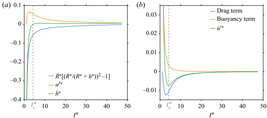
Figure 14. (a) Geometrical thinning term (first term on the right-hand side), entrainment term (second term on the right-hand side) and \dot{h}^* (left-hand side) in (5.3), as a function of time. (b) Buoyancy term (first term on the right-hand side), drag term (second term on the right-hand side) and \dot{u}^* (left-hand side) in (5.6), as a function of time. In this numerical solution, \rho_1/\rho_2 = 1.8 , Fr = 572 , \phi = 0.39 , \xi = 0.47 , \beta = 0.33 and C = 1.34 .
