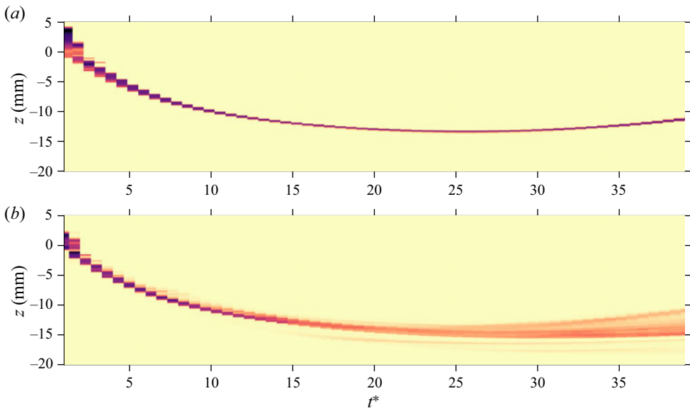
Figure 5. Composite images showing the LIF intensity as a function of vertical position and time, on the crater axis of symmetry ( \theta = 0 ). The two panels have been build from experiments without (a) ( \rho_1/\rho_2 = 1.0 ) and with (b) ( \rho_1/\rho_2 = 1.8 ) a density contrast between the drop and the pool. The surface of the pool prior to impact is at z = 0 .
