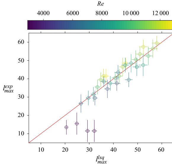
Figure 18. Experimental harmonic degree of maximum instability l_{max}^{exp} , as a function of the harmonic degree of maximum instability scaling l_{max}^{lsq} (A3). Colours scale as the Reynolds number Re .
