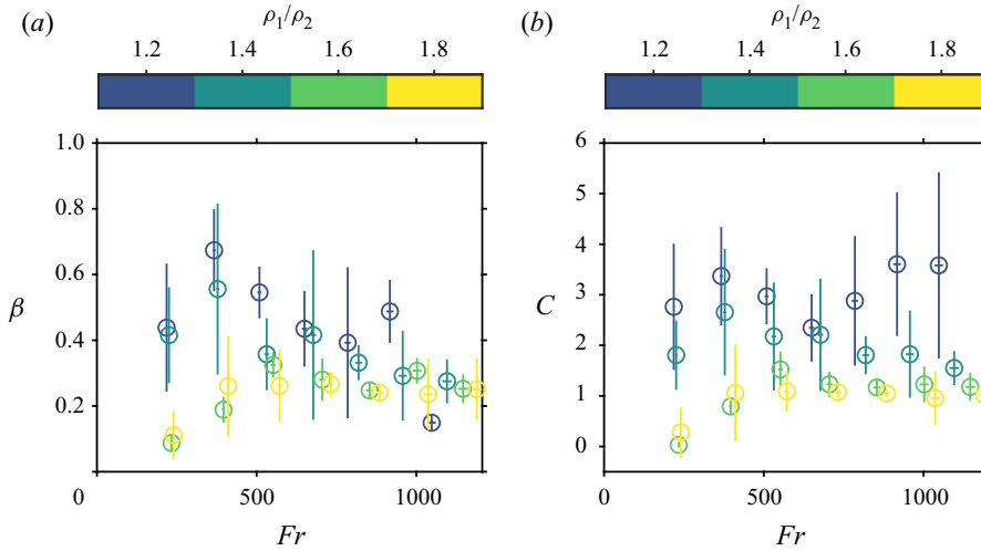
Figure 20. Buoyancy prefactor \beta (a), and drag coefficient C (b), as a function of the Froude number Fr . Colours scale as the density ratio \rho_1/\rho_2 .
