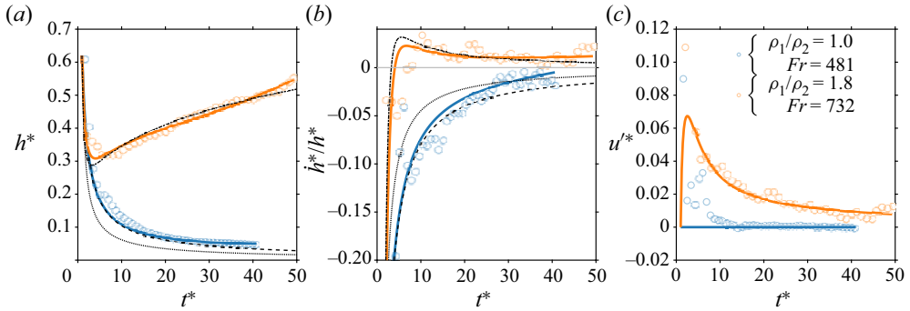
Figure 12. Time evolution of the normalised mixing layer thickness h^* (a), the normalised mixing layer growth rate \dot{h}^*/h^* (b) and the normalised inward flux due to entrainment u^{*} (estimated from (5.3)) (c), for two impact parameters with and without initial density difference. Circles and solid lines correspond, respectively, to experimental data and fitted buoyancy–drag model ((4.8), (5.3) and (5.6)). Dashed lines and dotted lines correspond, respectively, to the complete early-time power-law analytical solution (5.7) and the approximate early-time power-law analytical solution (5.9), calculated for the \rho_1/\rho_2 = 1.0 and Fr = 481 experiment. Dash–dotted lines correspond to the late-time power-law analytical solution (5.15 with h_0 = 0.62 , \dot{h}_0 = -1.14 and C = 0.71 ), calculated for the \rho_1/\rho_2 = 1.8 and Fr = 732 experiment.
