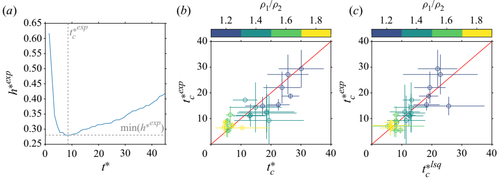
Figure 15. (a) Experimental mixing layer thickness h^{*exp} as a function of time, for a single experiment. The experimental transition time t_c^{*exp} between the thinning stage and the entrainment stage is defined as the time at which the mixing layer thickness reaches a local minimum. (b) Experimental transition time scale t_c^{*exp} as a function of the transition time t_c^* predicted by the buoyancy–drag model ((4.8), (5.3) and (5.6)). (c) Experimental transition time scale t_c^{*exp} as a function of the transition time scaling t_c^{*lsq} (5.19). Colours scale as the density ratio \rho_1/\rho_2 .
