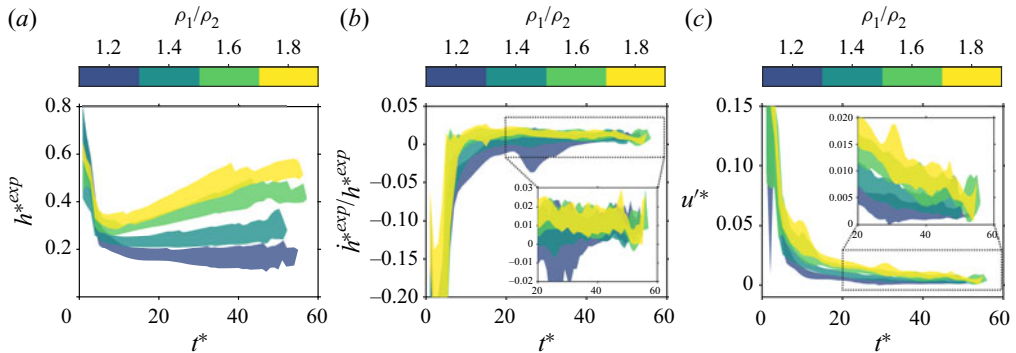
Figure 13. Time evolution of the experimental normalised mixing layer thickness h^{*exp} (a), the experimental mixing layer growth rate \dot{h}^{*exp}/h^{*exp} (b) and the normalised inward flux due to entrainment u^{*} (c) (estimated from (5.3)). Experiments are clustered by density ratio group, the extent of which is defined by the standard deviation of the experiments in that group. Colours scale as the density ratio \rho_1/\rho_2 .
