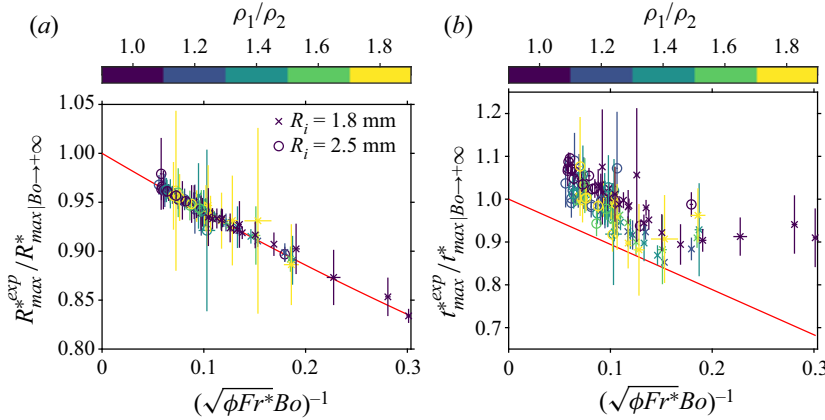
Figure 9. (a) Experimental maximum crater radius normalised by the maximum crater radius scaling without surface tension R_{max}^{*exp}/R_{max}^*|_{Bo \rightarrow +\infty} (4.14), as a function of 1/(\sqrt{\phi Fr^* Bo}) . The solid line corresponds to the surface tension correction of (4.19). (b) Experimental crater opening time normalised by the crater opening time scaling without surface tension t_{max}^{*exp}/t_{max}^*|_{Bo \rightarrow +\infty} (4.17), as a function of 1/(\sqrt{\phi Fr^* Bo}) . The solid line corresponds to the surface tension correction of (4.22). Colours scale as the density ratio \rho_1/\rho_2 . Circles and crosses correspond, respectively, to large and small drop size series.
