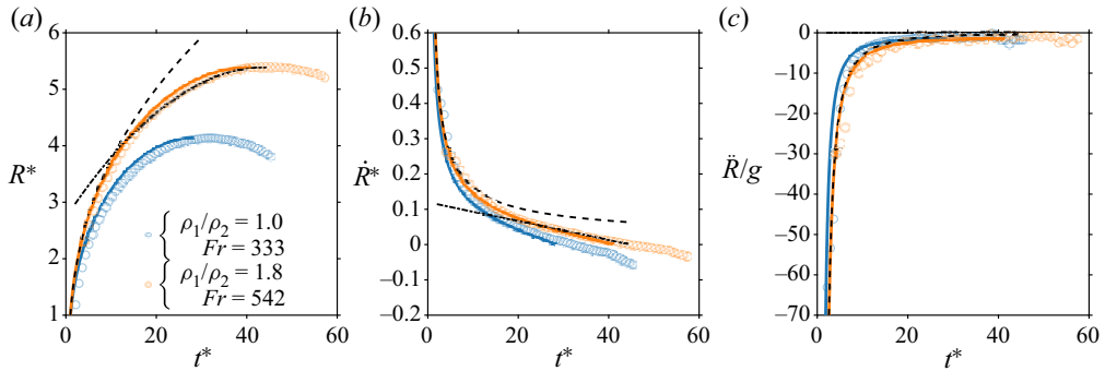
Figure 7. Time evolution of the normalised mean crater radius R^* (a), the normalised mean crater velocity \dot{R}^* (b) and the mean crater acceleration \ddot{R} normalised by the acceleration of gravity g (c), for two impact parameters. Circles and solid lines correspond, respectively, to experimental data and fitted energy model (4.8). Dashed lines and dashed–dotted lines correspond, respectively, to early-time power-law solution (4.10) and late-time quadratic solution (4.13) with \rho_1/\rho_2 = 1.8 and Fr = 542 .
