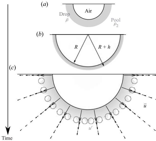
Figure 11. Mixing layer evolution. After having spread quickly on the crater boundary to become a thick layer(a), the liquid layer of the drop gradually gets thinner as the crater grows (b). At some point, crater expansion becomes weak enough, allowing for the RT instability to develop (c). We decompose the velocity field into a velocity component \bar{u} produced by crater opening, and velocity fluctuations u' produced by the RT instability.
