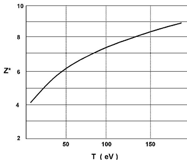
Fig. 6. Dependence of the average ionization from the temperature, according to the model of Lee and More (1984).
