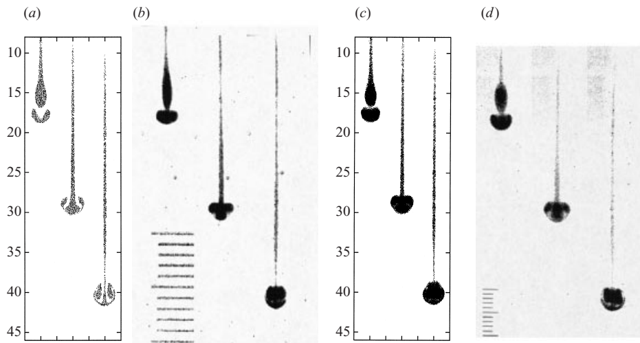
FIGURE 25. Quantitative comparison of computer simulations and experiments. (a) Computed drop positions in a sectional plane (parameter set C2 in table 2), \Delta t = 9.2 (equivalent to 3 s). (b) Corresponding photographs of drop positions from an experiment (same parameters, set E7 in table 3). (c) X/Z projection of computed drop positions (parameter set C5), \Delta t = 9.2 (equivalent to 13.5 s). (d) Corresponding photographs of drop positions from an experiment with the same parameters, set E9 in table 3. The scale bar in (b) and (d) shows 10 mm.
