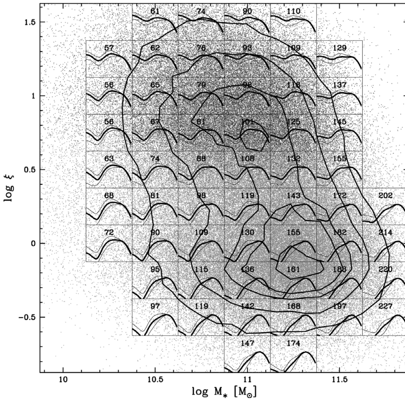
Figure 4. SFHs across the M_* versus \xi diagram for galaxies classified as AGN according to the \log[\text{N II}]/\text{H}\alpha > -0.40 criterion (S06 T in Figure 2d). The SFH curves are on the same scale as in Figure 3. Sources with W_{\text{H}\alpha} > 6 \text{ \AA} (Seyferts in the EW \alpha n2 diagram) are painted in black. Numbers within each box represent the median \sigma_* (in \text{km s}^{-1} ), believed to be a tracer of black-hole mass. Notice the bimodality in the \xi distribution. \xi \sim 1 indicates galaxies whose \text{H}\alpha luminosity can be entirely powered by its old stars, as in the retired galaxy model of S08. The SFH of galaxies in the \xi \sim 1 peak show that these systems have indeed stopped forming stars long ago.
