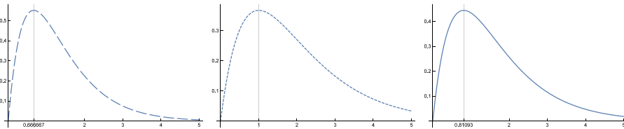
Figure 5. The pdf \tilde{f}_1(x) = f_{w_1 v_1}(x) (left part – dashed line), \tilde{f}_2(x) = f_{w_2 v_2}(x) (center part - dotted line), and \tilde{f}_3(x) = f_{w_3 v_3}(x) (right part – solid line) given in Example 3.1 for b = 2, \lambda = 1, \gamma = 0.5 , and 0 \leq x \leq 5 .
