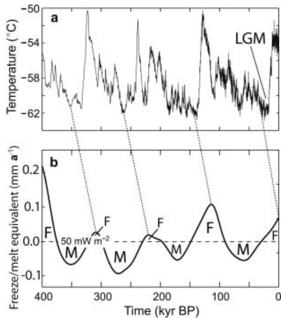
Fig. 7. Assumed surface forcing and calculated subglacial response based on thermal modelling of a 4100 m ice column above Lake Concordia. (a) Surface temperature variations derived from deuterium record in Vostok ice core adjusted so that the present surface temperature coincides with that at Dome C (Petit and others, 2000). (b) Calculated variation in basal melting/freezing rate (solid line) associated with heat flow from Lake Concordia into the base of the ice column compared with the basal melting rates associated with a geothermal heat flux of 50 \text{ mW m}^{-2} (dashed line). The net rate of freezing or melting resulting from these two processes is the difference between the geothermal contribution and the conductive loss. If the geothermal flux were 50 \text{ mW m}^{-2} the corresponding meltwater equivalent melting rate would be 4.75 \text{ mm a}^{-1} and a cyclic variation of net melting and net freezing would result. F: freezing; M: melting; LGM: Last Glacial Maximum. The dotted lines link the glacial minimum observed in the Vostok record with the resulting basal freezing.
