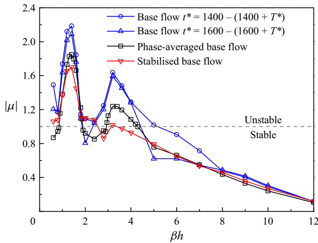
Figure 16. The |\mu|-\beta relationships for Re = 300 , predicted through the Floquet analysis using different base flows. The horizontal dashed line marks the neutral instability of |\mu| = 1.0 .
