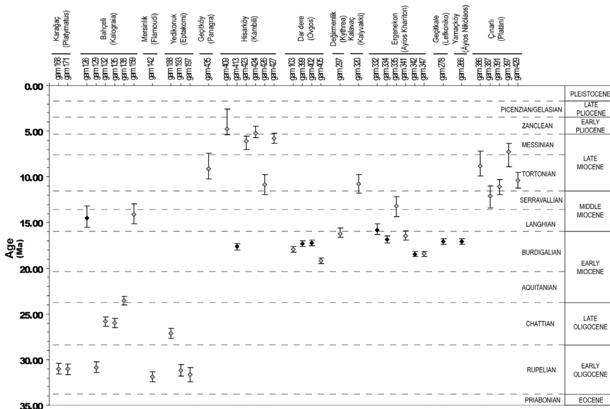
Figure 6. Results of 87 Sr/ 86 Sr analysis including error bars (calculated from empirical and analytical errors) and stages of deposition, plotted against the stages of sediment deposition. Sample numbers are arranged by locality (see Fig. 4). Black diamonds indicate samples that are found to be inconsistent with well-constrained biostratigraphic ages (see Tables 2 & 3). Note: owing to scaling, the data point for one sample (GAM 251) is not displayed to allow the error bars of other samples to be seen clearly. It should be noted that for the Sr isotopic dating method to work it is necessary to know the approximate age of the rocks in advance, a condition that is met in this case by the available biostratigraphical studies.
