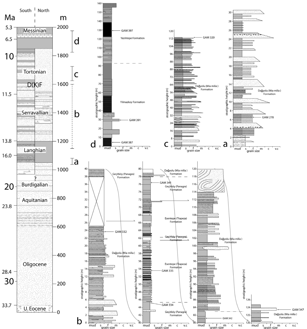
Figure 9. Composite sedimentary log of the Upper Eocene – Upper Miocene sedimentary rocks of the Değirmelik (Kythrea) Group as in Figure 8. Samples dated from the higher levels of the Upper Eocene – Upper Miocene Değirmelik (Kythrea) Group are shown on the following detailed sedimentary logs: (a) Geçitköy (Lefkoniko); (b) Ergenekon (Ayios Khariton); (c) Kalavaç (Kalyvacki); (d) stream section on ‘gypsum hill’ between Çınarlı (Platani) and Altınova (Áyios Iákovos). For legend, please see Figure 8. Locations are shown in Figure 4.
