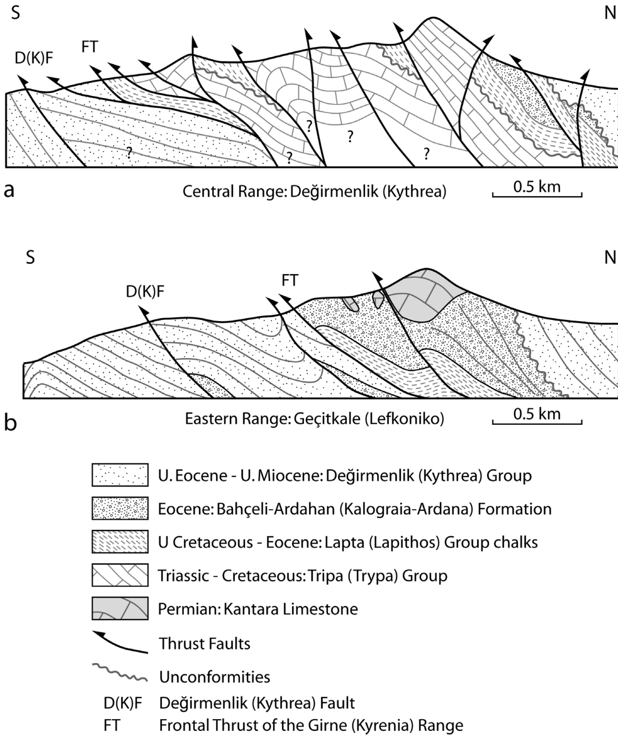
Figure 2. Simplified cross-sections of the Girne (Kyrenia) Range. (a) Western/central Girne (Kyrenia) Range; (b) eastern range. In contrast to further west, the eastern part of the range lacks an axial zone of Mesozoic platform carbonates, while sedimentary melange ('olistostromes') of the Eocene Bahçeli-Ardahan (Kalograia-Ardana) Formation is extensively exposed beneath the Upper Eocene-Upper Miocene Değirmenlik (Kythrea) Group. Modified from Baroz (1979) and Robertson & Woodcock (1986). The sections demonstrate the difficulty in sampling long intact sedimentary successions within this thrust belt.
