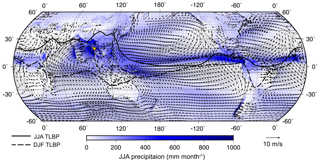
Figure 1 Global map showing the location of our sampling site (orange circle) and climatological components. The long-term (1950–2019 CE) mean surface wind vectors and precipitation ( \text{mm month}^{-1} ) for the June–August period are represented by arrows and blue shading, respectively, and were derived from the ERA5 dataset (Hersbach et al. 2020). The mean positions of the TLBP during June–August (JJA: solid line) and December–February (DJF: dashed line) were derived from Hua et al. (2022) and are based on the NCEP/NCAR sea level pressure data. (Please see online version for color figures.)
