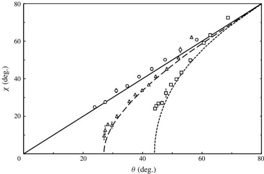
FIGURE 7. Experimental data for the beam angle \chi as a function of \theta set by the driving frequency \omega = \sin \theta , for tilt angle \phi = 0^\circ ( \circ ), \phi = 27^\circ ( \Delta ) and \phi = 44^\circ ( \square ); the corresponding theoretical curves, obtained by (2.5), are included as solid, dashed and dotted lines, respectively. The error bars are the standard deviation of the mean.
