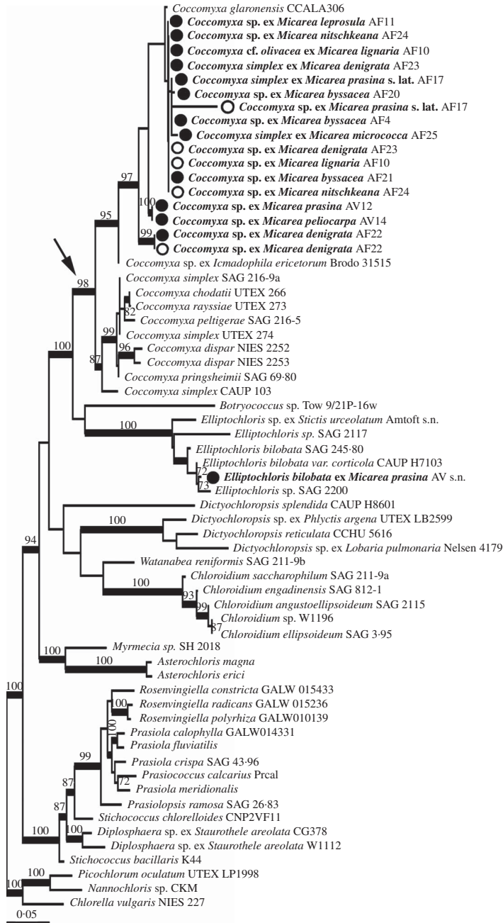
FIG. 2. Maximum likelihood phylogeny from combined rbclL and nucSSU of Micarea photobionts. Morphological determinations of studied strains are labelled on the terminals according to Micarea species with which they were associated, and the collection code for the specimen. Bootstrap support is shown above nodes for values above 70%. Support for nodes from ML analysis but without support from BI is shown to the right of nodes. Thickened branches indicate support over 0.97 in BI. Terminal names in bold show strains studied here. Open circles depict sequences derived from direct amplification of algae from fresh material, closed circles for photobionts sequenced from cultures and arrow indicates the Coccomyxa clade.
