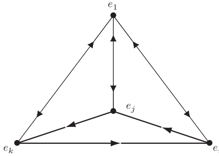
Fig. 1. Suspension trick: the cycle e_i \wedge e_j + e_j \wedge e_k + e_k \wedge e_i is equal to the boundary (e_1 \wedge e_i \wedge e_j)\delta_3 + (e_1 \wedge e_j \wedge e_k)\delta_3 + (e_1 \wedge e_k \wedge e_i)\delta_3 .
