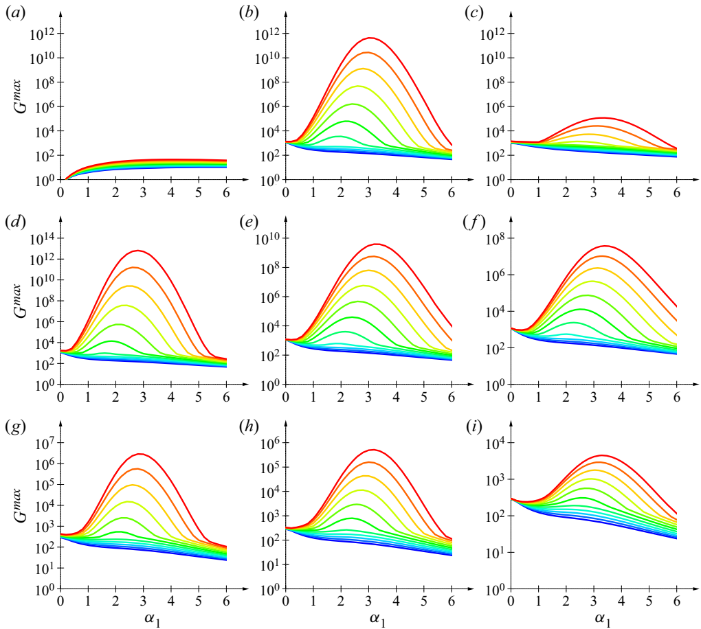
Figure 16. Maximum energy growth G^{max} for pulsating pipe flows, over 0 < \alpha_1 < 6 at \tilde{Q} = 0.0, 0.1, 0.2, \dots, 1.0 . Here (a–f) Re = 4000 and (g–i) Re = 2000 ; (a–c,h) Wo = 10 , (d,g) Wo = 8 , (e) Wo = 12 and (f,i) Wo = 14 ; (a) \alpha_2 = 0 , (b,d–i) \alpha_2 = 1 and (c) \alpha_2 = 2 .
