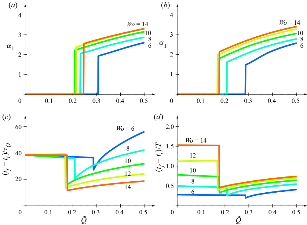
Figure 19. Characterisation of the maximally amplified optimal perturbations as the pulsation amplitude \tilde{Q} is increased for W_o = 6, 8, 10, 12, 14 . Streamwise wavenumber \alpha_1 at (a) Re = 2000 and (b) Re = 4000 . Duration of transient growth t_f - t_i at Re = 4000 (c) measured in mean-flow advection units \tau_Q and (d) in pulsation periods T .
