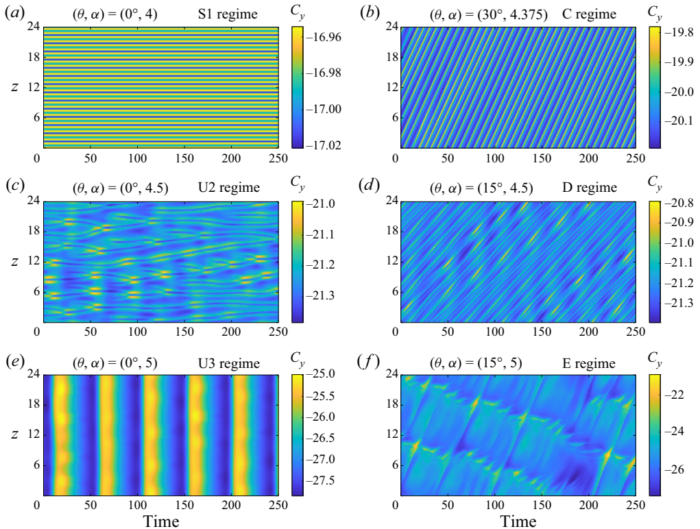
Figure 3. Selected time series of the CF force coefficient along the span for (a) (\theta, \alpha) = (0^\circ, 4) , (b) (\theta, \alpha) = (30^\circ, 4.375) , (c) (\theta, \alpha) = (0^\circ, 4.5) , (d) (\theta, \alpha) = (15^\circ, 4.5) , (e) (\theta, \alpha) = (0^\circ, 5) and (f) (\theta, \alpha) = (15^\circ, 5) . Flow regime is specified in each panel.
