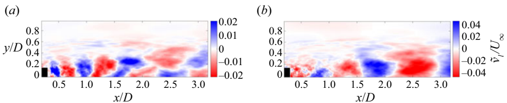
Figure 5. Transverse velocity components of the OMD modes associated with frequencies (a) f_n and (b) f_{wm} for \lambda = 5.5 obtained from experiment 1B.
