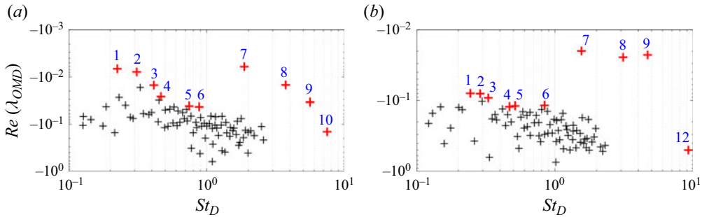
Figure 2. The OMD spectra obtained for (a) \lambda = 6 and (b) \lambda = 5 from experiment 1A. The modes shown by a red + sign are selected for a lower-order representation of the flow. The high-frequency modes with St_D > 1 are related to the tip vortices. The low-frequency modes ( St_D < 1 ) are associated with wake meandering, and the sheddings from the nacelle and the tower.
