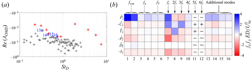
Figure 19. (a) The OMD spectrum for \lambda = 6 from experiment 1A. The ‘blue \circ ’ symbols show the additional low-frequency modes ( St_D < 1 ) retained. Panel (b) shows the energy budget terms of (4.1) summed over the domain of investigation for all the modes including the additional low-frequency modes.
