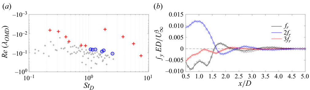
Figure 20. (a) The OMD spectrum for \lambda = 6 from experiment 1A. The ‘blue \circ ’ symbols show the additional modes retained in the range 1 \lesssim St_D \lesssim 3 . Plot (b) shows the streamwise evolution of the spanwise-averaged net triadic energy production term for f_r - 3f_r with (circles) and without (solid lines) the inclusion of the additional modes.
