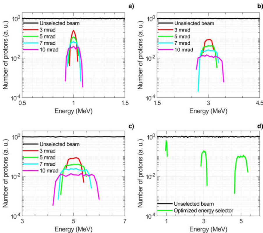
Fig. 2. Final energy spread as function of the initial divergence, for the case of 1 MeV (a), 3 MeV (b), and 5 MeV (c), at the exit of the selector. The initial divergence has the values: 3 mrad (red color), 5 mrad (green color), 7 mrad (light blue color), 10 mrad (magenta color). The dark black curve represents the unselected beam at the entrance of the selector. (d) Final energy spectra in the case of 1, 3, and 5 MeV beams, selected using 5 mrad and a_2 = 1000 \mu\text{m} (1 MeV beam), and 3 mrad and a_2 = 500 \mu\text{m} (3 and 5 MeV beams).
