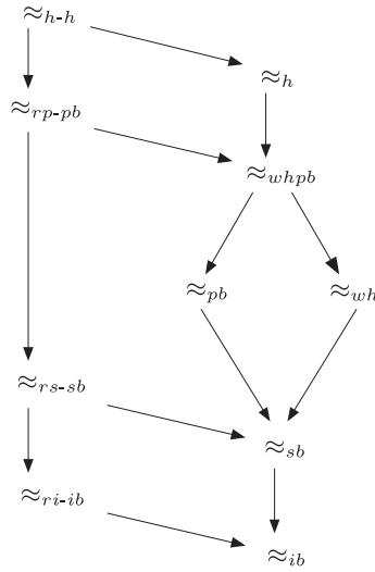
Fig. 25. The hierarchy of main bisimulations.
