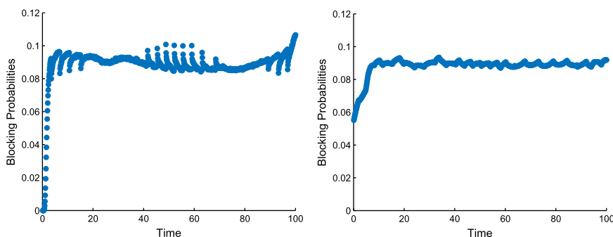
FIGURE 10. (Colour online) Simulation estimates of the blocking probabilities in the non-stationary M_t/M/s_t/0 model with parameter triple (20, 5, 100) having average arrival rate \bar{\lambda} = 20 with the staffing algorithm for target B = 0.1 using randomization with \sigma = 3.84 (left) and averaging with \Delta = 9.6 (right).
