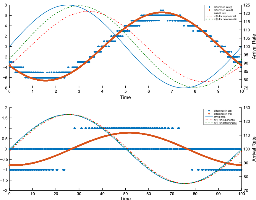
FIGURE 30. (Colour online) The difference between the staffing functions for the M_t/M/s_t/0 and M_t/D/s_t/0 models with the sinusoidal arrival rate in (5.1) and mean-1 exponential and deterministic service-time distributions and parameter four-tuples (\bar{\lambda}, \beta, T, B) = (100, 25, T, 0.1) for T = 10 (top) and T = 100 (bottom).
