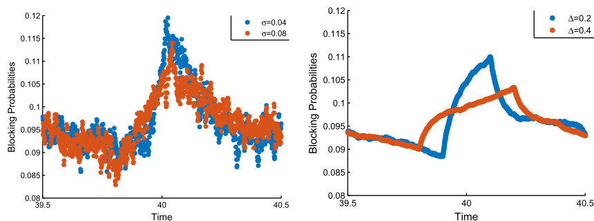
FIGURE 7. (Colour online) A careful examination of the time interval [39.5, 40.5] in the setting of Figure 6: randomization for \sigma = 0.04 and 0.08 (left) and averaging for \Delta = 0.2 and 0.4 (right).
