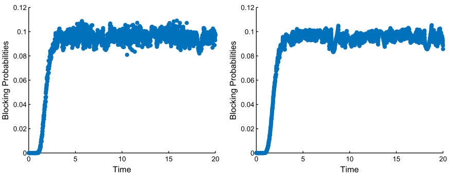
FIGURE 21. (Colour online) Simulation estimates of the blocking probabilities in the non-stationary M_t/M/s_t/0 model with parameter triple (100, 25, 10) having average arrival rate \bar{\lambda} = 100 with the staffing algorithm for target B = 0.1 using randomization with averaging parameters \sigma = 0.08 (left) and \Delta = 0.20 (right).
