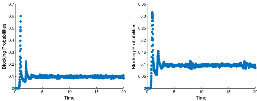
FIGURE 29. (Colour online) Simulation estimates of the blocking probabilities in the non-stationary M_t/D/s_t/0 model with parameter triple (100, 25, 10) having average arrival rate \bar{\lambda} = 100 with the staffing algorithm for target B = 0.1 using randomization with \sigma = 0.08 (left) and averaging with \Delta = 0.2 (right).
