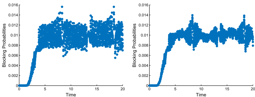
FIGURE 24. (Colour online) Simulation estimates of the blocking probabilities in the non-stationary M_t/M/s_t/0 model with parameter triple (100, 25, 10) having average arrival rate \bar{\lambda} = 100 with the staffing algorithm for target B = 0.01 using randomization with too small averaging parameters \Delta = 0.04 (left) and \Delta = 0.08 (right).
