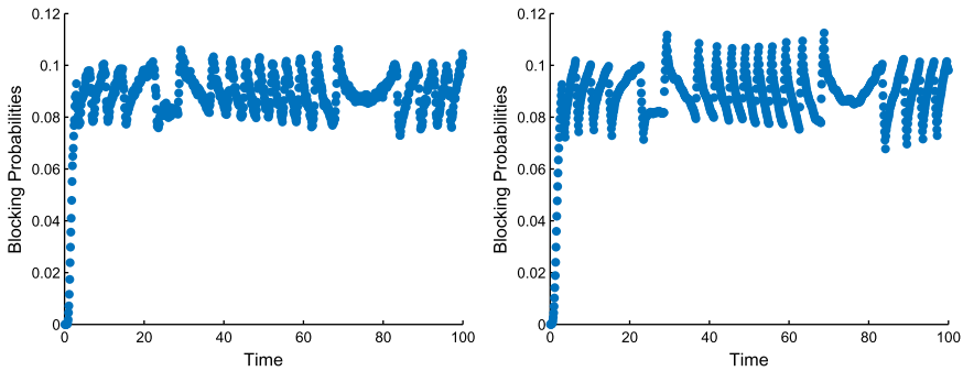
FIGURE 9. (Colour online) Simulation estimates of the blocking probabilities in the non-stationary M_t/M/s_t/0 model with parameter four-tuple (20, 5, 100, 0.1) having average arrival rate \bar{\lambda} = 20 using randomization with \sigma = 0.32 (left) and averaging with \Delta = 0.8 (right).
