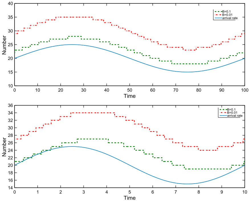
FIGURE 3. (Colour online) The MOL staffing functions and the sinusoidal arrival rate function in (5.1) for the M_t/M/s/0 model with \mu = 1 , average arrival rate \bar{\lambda} = 20 , amplitude \beta = 5 , and two blocking probability targets B = 0.1 and 0.01 : for long cycles T = 100 (top) and short cycles T = 10 (bottom).
