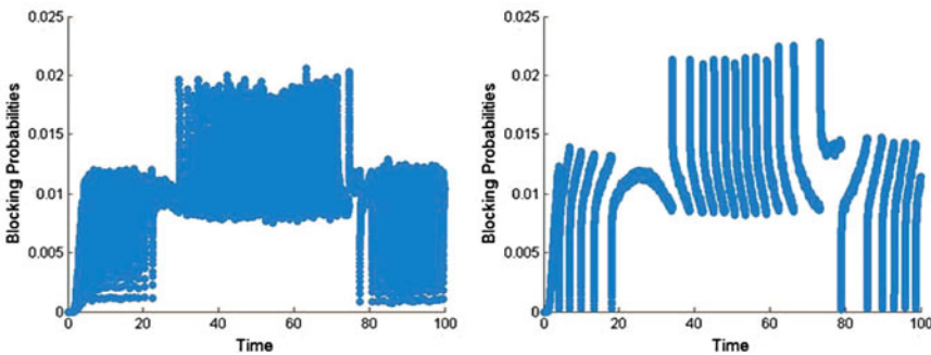
FIGURE 12. (Colour online) Simulation estimates of the blocking probabilities in the non-stationary M_t/M/s_t/0 model with the staffing algorithm without any averaging, for the sinusoidal arrival rate in (5.1) and parameter triple (100, 25, 100, 0.01) (left) and (20, 5, 100, 0.01) (right).
