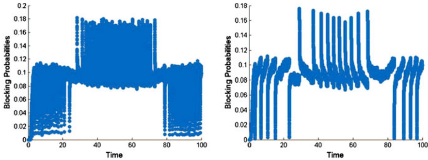
FIGURE 5. (Colour online) Simulation estimates of the blocking probabilities in the non-stationary M_t/M/s_t/0 model with the staffing algorithm without any averaging, for the sinusoidal arrival rate in (5.1) and parameter triple (100, 25, 100, 0.1) (left) and (20, 5, 100, 0.1) (right).
