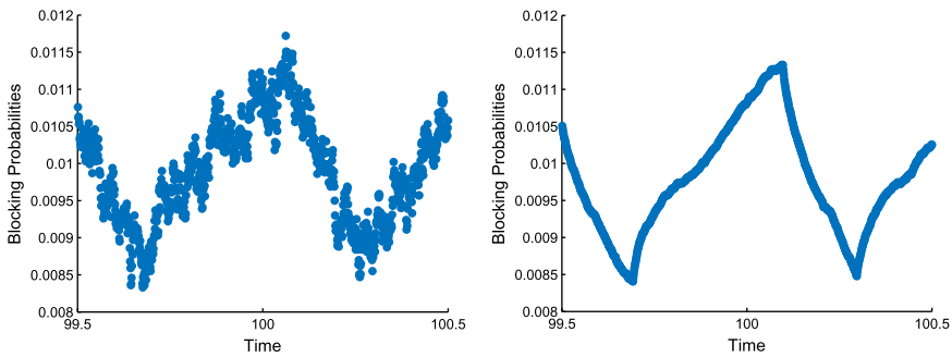
FIGURE 15. (Colour online) A careful examination of the time interval [99.5, 100.5] for the case (100, 25, 100, 0.01) in the setting of Figure 13: randomization for \sigma = 0.08 (left) and averaging for \Delta = 0.2 (right).
