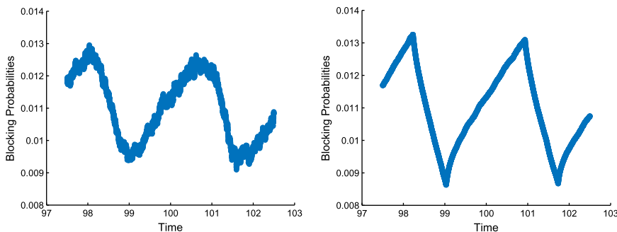
FIGURE 19. (Colour online) A careful examination of the time interval [97.5, 102.5] for the case (20, 5, 100) in the setting of Figure 17: randomization for \sigma = 0.32 (left) and averaging for \Delta = 0.8 (right).
