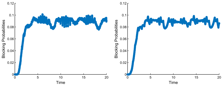
FIGURE 26. (Colour online) Simulation estimates of the blocking probabilities in the non-stationary M_t/M/s_t/0 model with parameter triple (20, 5, 10) having average arrival rate \bar{\lambda} = 20 with the staffing algorithm for target B = 0.1 using randomization with averaging parameters \sigma = 0.32 (left) and \Delta = 0.80 (right).
