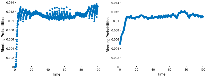
FIGURE 20. (Colour online) Simulation estimates of the blocking probabilities in the non-stationary M_t/M/s_t/0 model with parameter triple (20, 5, 100) having average arrival rate \bar{\lambda} = 20 with the staffing algorithm for target B = 0.01 using randomization with \sigma = 3.84 (left) and averaging with \Delta = 9.60 (right).
