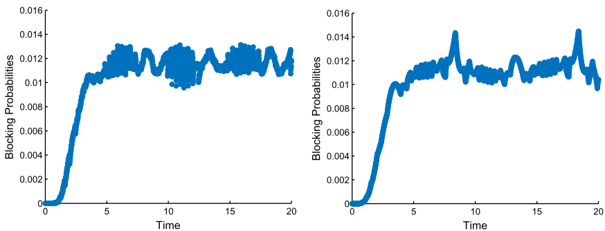
FIGURE 27. (Colour online) Simulation estimates of the blocking probabilities in the non-stationary M_t/M/s_t/0 model with parameter triple (20, 5, 10) having average arrival rate \bar{\lambda} = 20 with the staffing algorithm for target B = 0.01 using randomization with averaging parameters \sigma = 0.32 (left) and \Delta = 0.80 (right).
