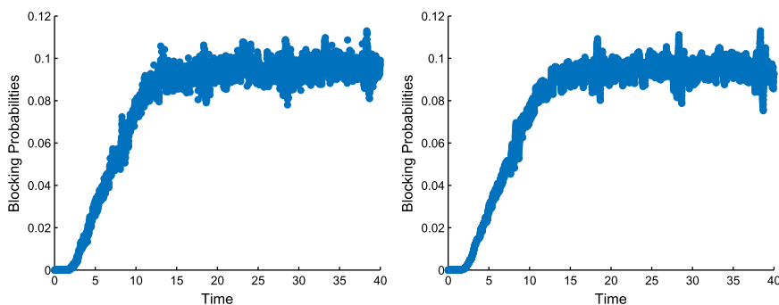
FIGURE 28. (Colour online) Simulation estimates of the blocking probabilities in the non-stationary M_t/H_2/s_t/0 model with parameter triple (100, 25, 10) having average arrival rate \bar{\lambda} = 100 with the staffing algorithm for target B = 0.1 using randomization with \sigma = 0.08 (left) and averaging with \Delta = 0.2 (right).
