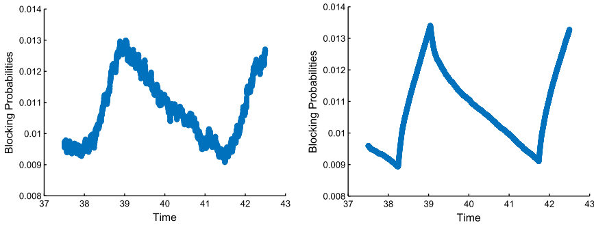
FIGURE 18. (Colour online) A careful examination of the time interval [37.5, 42.5] for the case (20, 5, 100, 0.01) in the setting of Figure 17: randomization for \sigma = 0.32 (left) and averaging for \Delta = 0.8 (right).
