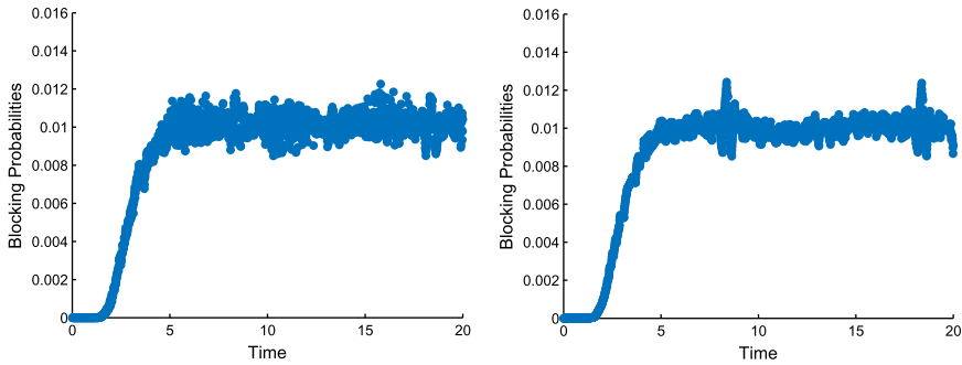
FIGURE 22. (Colour online) Simulation estimates of the blocking probabilities in the non-stationary M_t/M/s_t/0 model with parameter triple (100, 25, 10) having average arrival rate \bar{\lambda} = 100 with the staffing algorithm for target B = 0.01 using randomization with averaging parameters \sigma = 0.08 (left) and \Delta = 0.20 (right).
