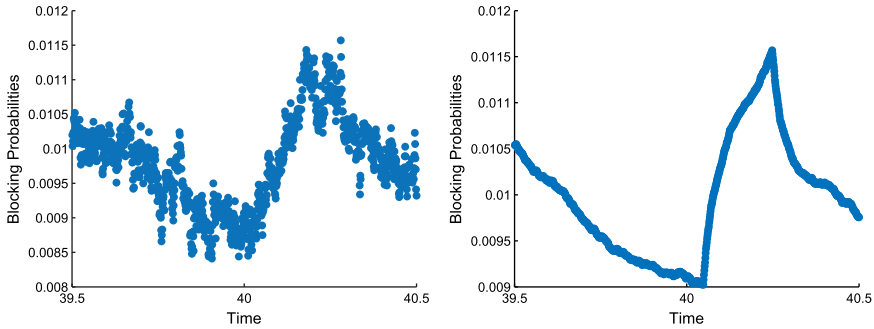
FIGURE 14. (Colour online) A careful examination of the time interval [39.5, 40.5] for the case (100, 25, 100, 0.01) in the setting of Figure 13: randomization for \sigma = 0.08 (left) and averaging for \Delta = 0.2 (right).
