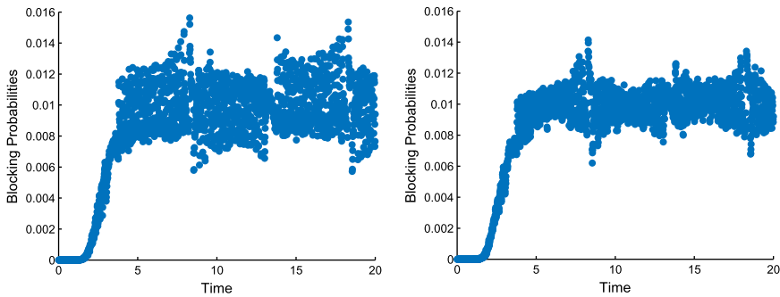
FIGURE 23. (Colour online) Simulation estimates of the blocking probabilities in the non-stationary M_t/M/s_t/0 model with parameter triple (100, 25, 10) having average arrival rate \bar{\lambda} = 100 with the staffing algorithm for target B = 0.01 using randomization with too small averaging parameters \sigma = 0.01 (left) and \sigma = 0.02 (right).
