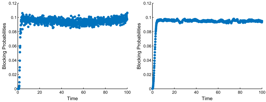
FIGURE 8. (Colour online) Simulation estimates of the blocking probabilities in the non-stationary M_t/M/s_t/0 model with parameter triple (100, 25, 100) having average arrival rate \bar{\lambda} = 100 with the staffing algorithm for target B = 0.1 using randomization with \sigma = 0.96 (left) and averaging with \Delta = 2.4 (right).
