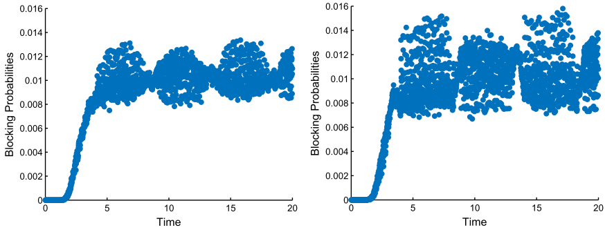
FIGURE 25. (Colour online) Simulation estimates of the blocking probabilities in the non-stationary M_t/M/s_t/0 model with parameter triple (100, 25, 10) having average arrival rate \bar{\lambda} = 100 with the staffing algorithm for target B = 0.01 using randomization with too large averaging parameters \sigma = 0.20 (left) and \sigma = 2.0 (right).
