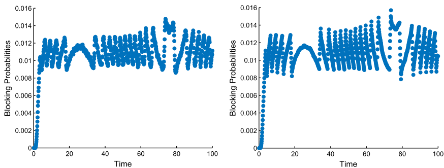
FIGURE 17. (Colour online) Simulation estimates of the blocking probabilities in the non-stationary M_t/M/s_t/0 model with parameter four-tuple (20, 5, 100, 0.01) using randomization with \sigma = 0.32 (left) and averaging with \Delta = 0.8 (right).
