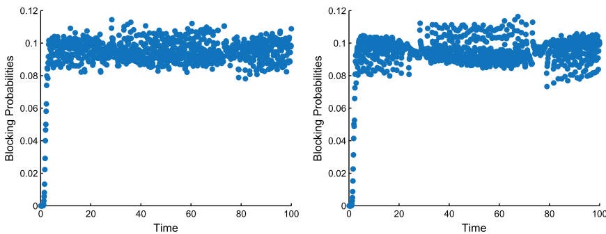
FIGURE 6. (Colour online) Simulation estimates of the blocking probabilities in the non-stationary M_t/M/s_t/0 model with parameter triple (100, 25, 100) having average arrival rate \bar{\lambda} = 100 with the staffing algorithm for target B = 0.1 using randomization with \sigma = 0.08 (left) and averaging with \Delta = 0.2 (right).
