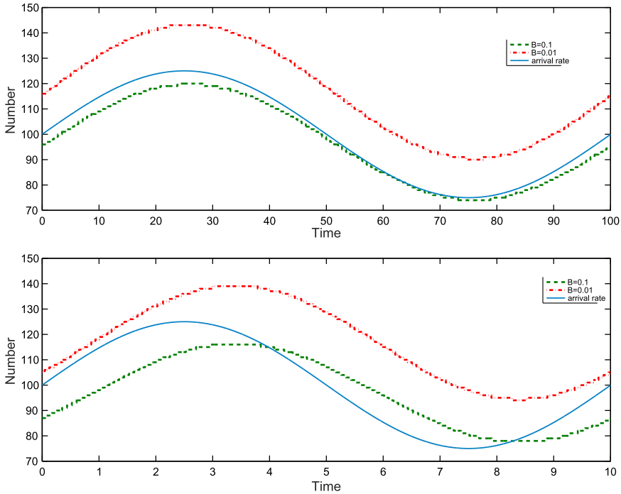
FIGURE 2. (Colour online) The MOL staffing functions and the sinusoidal arrival rate function in (5.1) for the M_t/M/s/0 model with \mu = 1 , average arrival rate \bar{\lambda} = 100 , amplitude \beta = 25 , and two blocking probability targets B = 0.1 and 0.01 : for long cycles T = 100 (top) and short cycles T = 10 (bottom).
