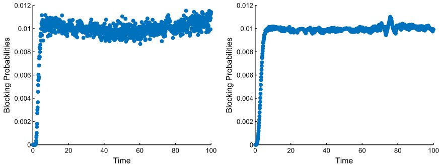
FIGURE 16. (Colour online) Simulation estimates of the blocking probabilities in the non-stationary M_t/M/s_t/0 model with parameter triple (100, 25, 100) having average arrival rate \bar{\lambda} = 100 with the staffing algorithm for target B = 0.01 using randomization with \sigma = 0.96 (left) and averaging with \Delta = 2.4 (right).
