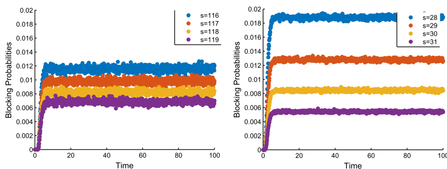
FIGURE 11. (Colour online) Simulation estimates of the blocking probabilities in the stationary M/M/s/0 model for arrival rate \lambda = 100 (left) and \lambda = 20 (right) with four different staffing levels yielding blocking above and below 0.01, showing the impact of a single server.
