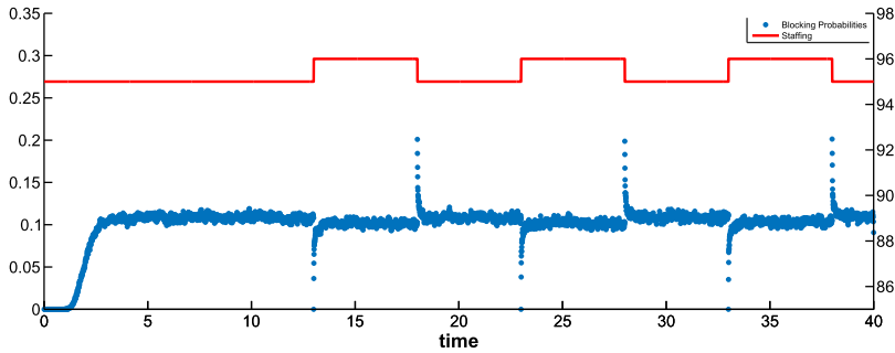
FIGURE 1. (Colour online) Simulation estimates of the time-varying blocking probabilities (left axis) with time-varying staffing (right axis) in an Erlang loss model with arrival rate \lambda = 100 and service rate \mu = 1 , starting empty, in response to six staffing changes.
