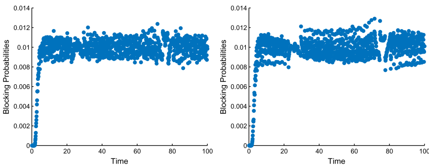
FIGURE 13. (Colour online) Simulation estimates of the blocking probabilities in the non-stationary M_t/M/s_t/0 model with parameter four-tuple (\bar{\lambda}, \beta, T, B) = (100, 25, 100, 0.01) using randomization with \sigma = 0.08 (left) and averaging with \Delta = 0.2 (right).
