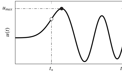
FIGURE 3. Solution of (3.17) near the turning point t_* ; the maximum is achieved after passing through t_* .
