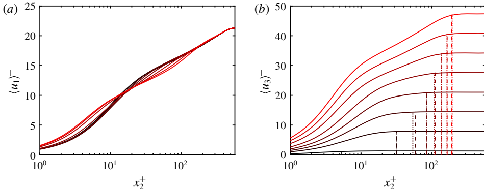
FIGURE 3. Mean velocity profile in (a) the streamwise direction and (b) the spanwise direction for t^+ = 12, 72, 132, 192, 252, 312, 372 and 432 . Colours indicate time from t^+ = 0 (black) to t^+ = 432 (red). The vertical dotted lines are the boundary layer thickness \delta_3 defined by the wall-normal distance at which \langle u_3 \rangle = 0.99 \langle u_3 \rangle_\infty = 0.99 \langle u_3 \rangle(h, t) , and the vertical dashed lines are the estimated boundary layer thickness given by \delta_3^+ = 0.445t^+ .
