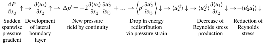
FIGURE 16. Summary of the sequential process of Reynolds stress reduction from the sudden imposition of a spanwise pressure gradient up to the final decrease in tangential Reynolds stress. Time goes from left to right. See text for details.
