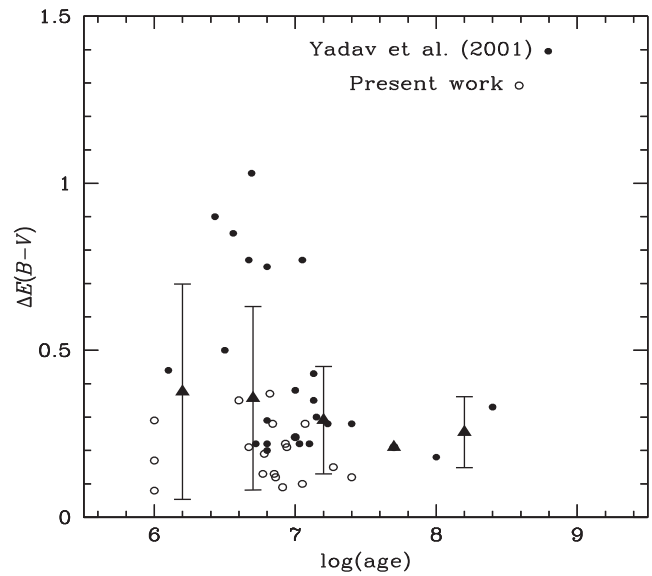
Figure 8. Variation of \Delta E(B - V) with the cluster age. The open circles denote data points from present work and the filled circles denotes data points from Yadav & Sagar (2001). Note: Error bars denote the corresponding standard deviation of binned data.
