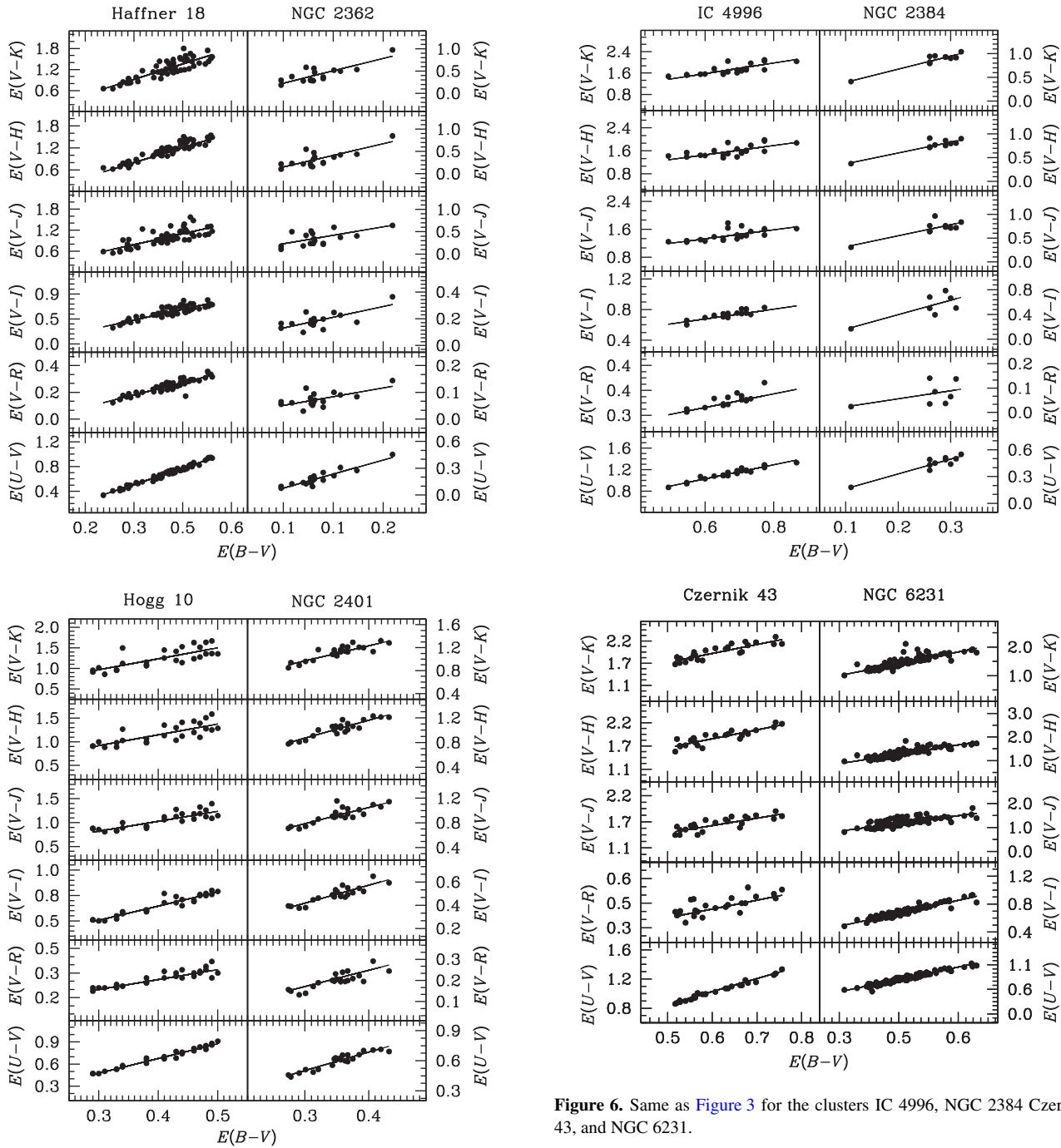
Figure 5. Same as Figure 3 for the clusters Haffner 18, NGC 2362, Hogg 10, and NGC 2401.
