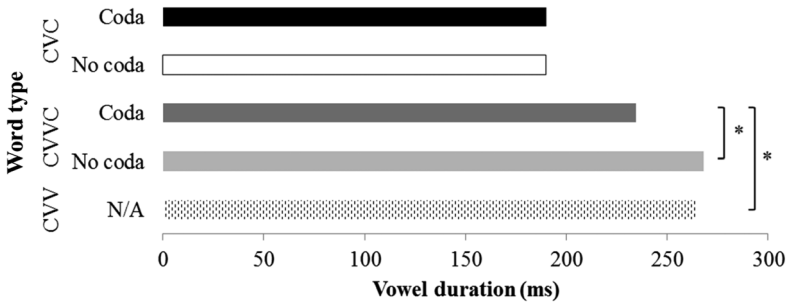
Fig. 6. Vowel durations as a function of condition and coda realisation ( *=p < .05 ).
