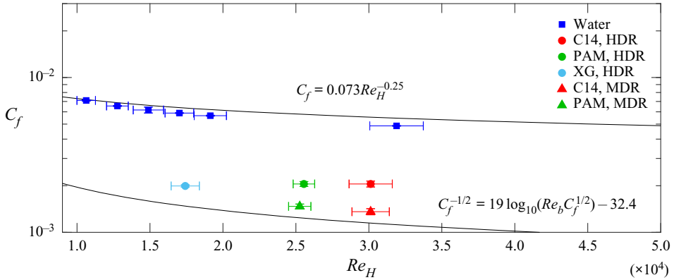
Figure 4. Skin-friction coefficient as a function of bulk Reynolds number for drag-reduced flows and water. The upper equation shows the Dean (1978) correlation for Newtonian channel flows and the lower equation shows the MDR asymptote adapted for channel flows.
