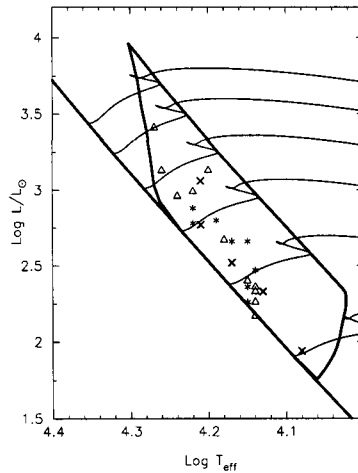
Figure 1. The position of the 24 SPBs (x: SPBs discovered by Waelkens (1991), \Delta : southern Hipparcos SPBs, *: northern Hipparcos SPBs) is confronted with the theoretical instability strip determined by Pamyatnykh (1999).
