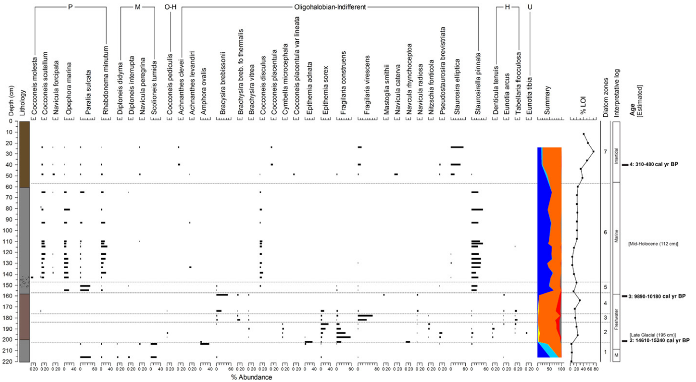
Figure 4. Diatom assemblage (species greater than 5% abundance shown), lithostratigraphy (see Fig. 3 for key), loss on ignition and interpretative log for Loch Duart Marsh (core LDM-13-1), illustrating the transition from marine to freshwater conditions between zone 1 and 2 and zone 4 and 5. The position and calibrated age of radiocarbon ages are shown as well as the age indicated by the supporting pollen analysis (Supplementary Table 1).
