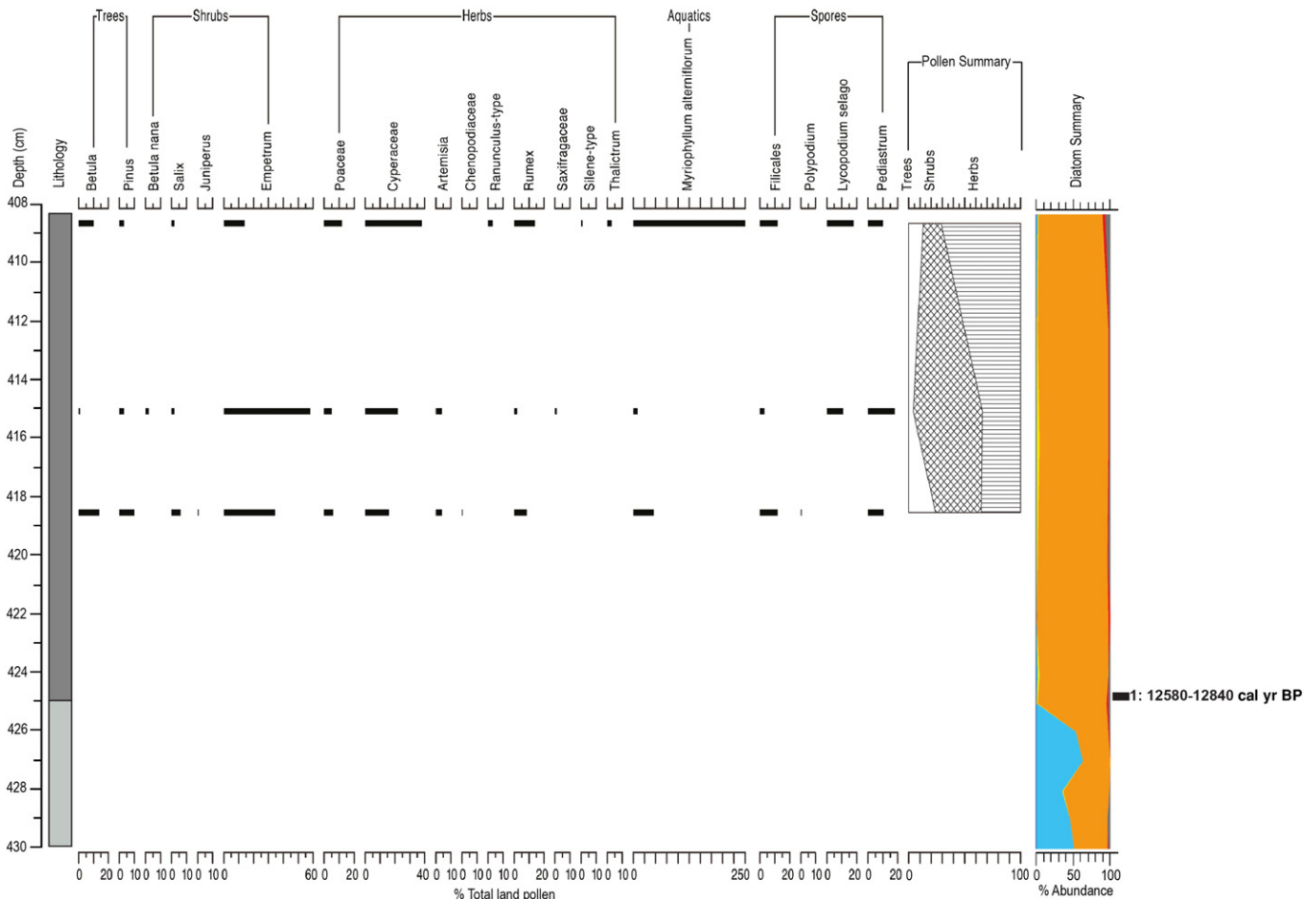
Figure 5. Summary pollen and diatom flora, lithostratigraphy (see Fig. 3 for key), pollen assemblage and calibrated radiocarbon age for Duart Bog (core DuB-13-3).
