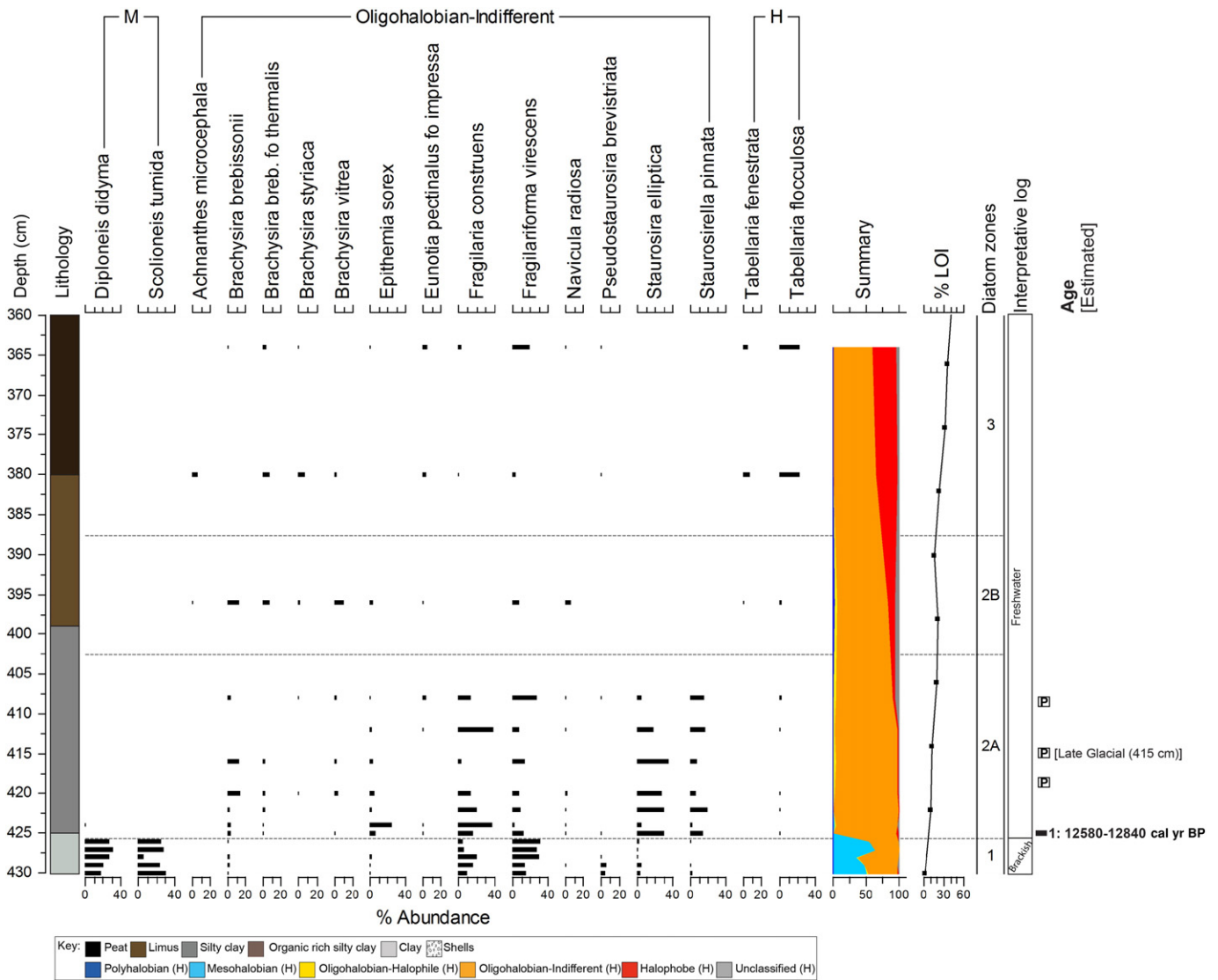
Figure 3. Diatom assemblage (species greater than 5% abundance shown), lithostratigraphy, loss on ignition and interpretative log for Duart Bog (core DuB-13-3), illustrating the transition from brackish-dominant to freshwater conditions between zone 1 and 2A. The position and calibrated age of radiocarbon ages are shown as well as the age indicated by the supporting pollen analysis (shown by the P) (Fig. 5).
