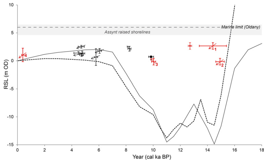
Figure 6. Sea-level curves from Bradley et al. (2011) (solid line) and Kuchar et al. (2012) (dashed line) model predictions for Assynt, including previous sea-level index points for the Assynt region from Coigach (Shennan et al., 2000), shown in black, and from Duart (this study), in red. Index point 1 (DuB-13-3) based on radiocarbon material is denoted by the red diamond symbol whilst limiting index points are denoted by a black square. The arrows indicate the positive (rising arrow) or negative (falling arrow) tendency associated with each sea-level index point.
