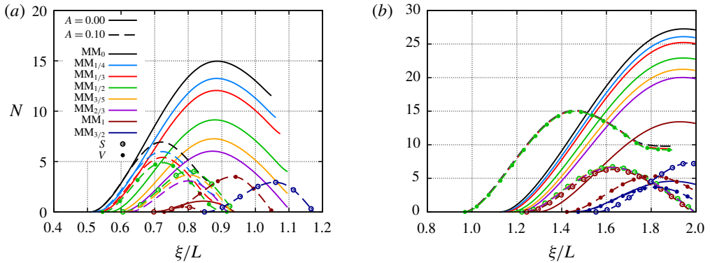
FIGURE 11. (Colour online) Evolution of N -factors with frequencies (a) \omega=0.603 and (b) \omega=0.421 of planar and selected oblique Mack-mode waves for the unperturbed boundary-layer flow ( A=0.00 ) and the perturbed boundary-layer flow with A=0.10 .
