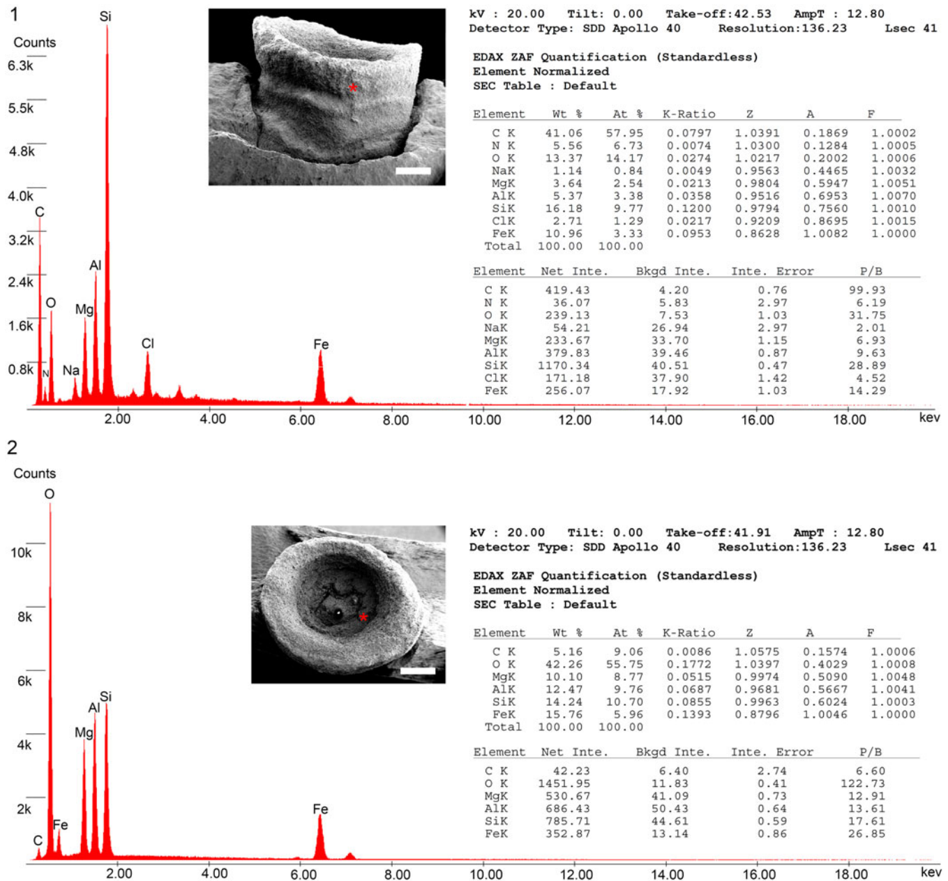
Figure 6. Wall composition of Anulitubus formosus n. gen. n. sp. Moczydlowska in Moczydlowska et al., holotype specimen PMU 34736, shown by elemental content analyzed by STEM EDS on the wall surface in (1) and the incomplete septum in (2). Measured points are marked by red asterisks. The point spectra are characteristic of silica forming the wall with high content of element carbon indigenous to the wall and remnant of organic matter.
