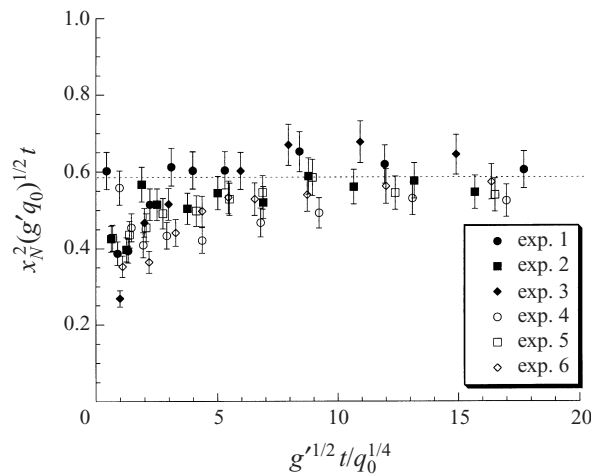
FIGURE 5. Ratio of the measured position of the leading edge of the current and the self-similar scaling for the position, x_N^2 / (g' q_0 t^2)^{1/2} , as a function of the dimensionless time g'^{1/2} t / q_0^{1/4} for experiments 1 to 6.
